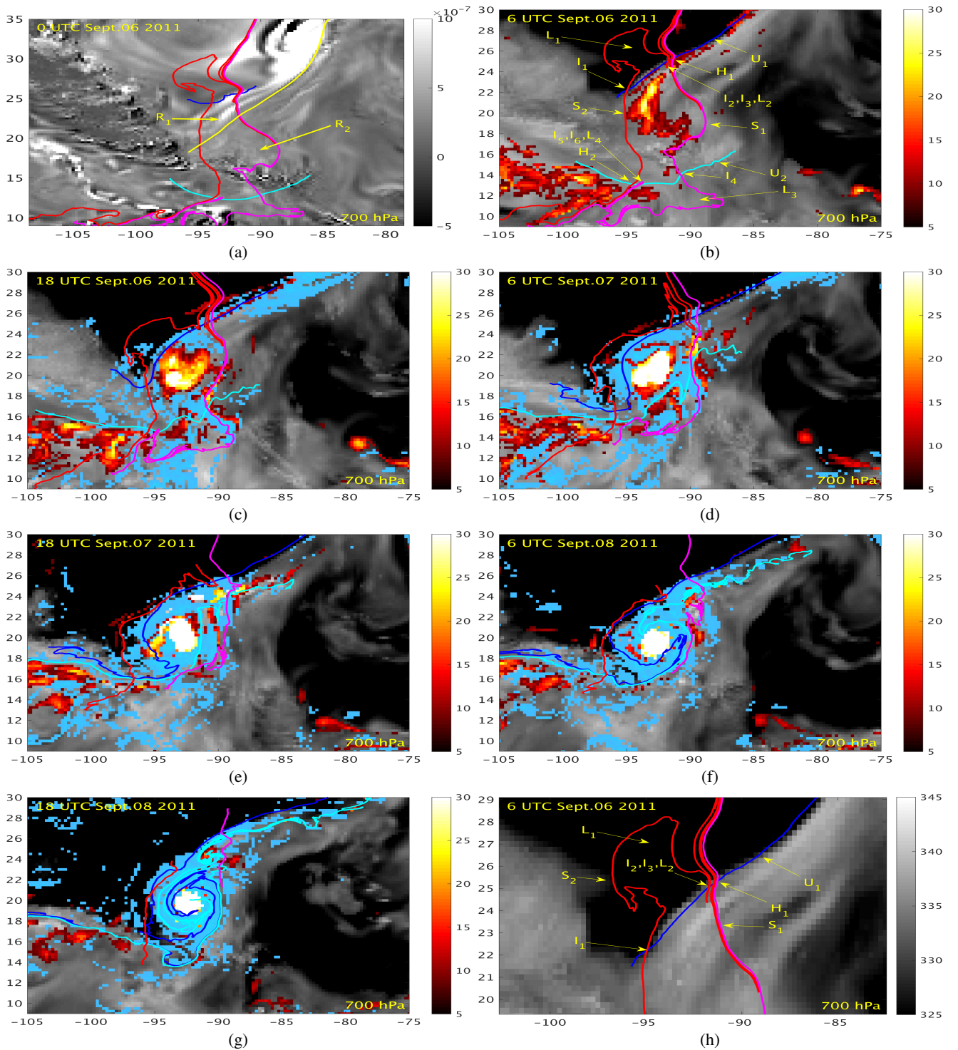
Figure 2. The stable (red, magenta) and unstable (blue, cyan) manifolds are overlaid on the ECMWF PV field ( M \cdot m^2 / kg \cdot s ) in (a) and \theta_e field (K) (background with gray colors) at 700 hPa in (b-g) showing the time-evolution of the manifolds from Sept. 6 to Sept. 8. The hot colormap shows the \zeta_{Lag} values while the cool colors indicate OW_{Lag} values of less than -8 indicating high strain. Labels are provided in panels (a) and (b). A zoom of the features that are shown in panel (b) is shown in panel (h), which also shows the colorbar for the \theta_e field. An attracting line from the Lee flow is shown in yellow in (a).
