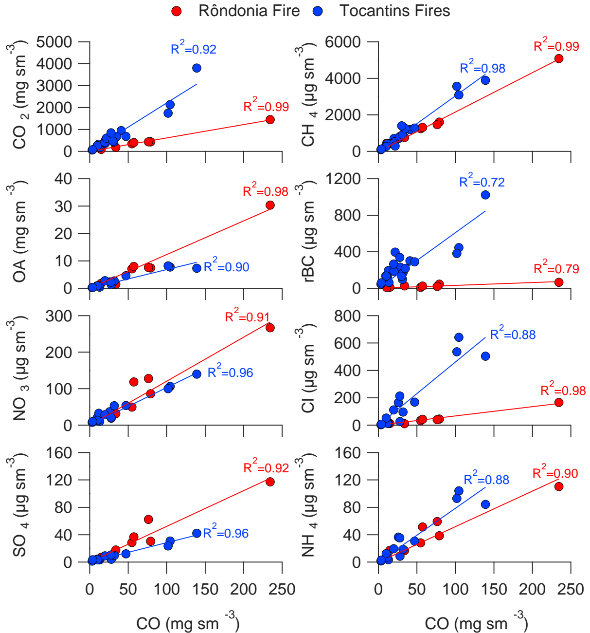
Figure 2. Relationship between excess concentrations of trace gas and particulate phase species relative to excess carbon monoxide for the R ndonia and Tocantins fires. Solid lines show line of best fit from linear regressions forced through zero.
