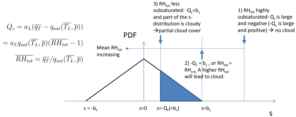
Figure A1. The assumed triangular shaped PDF, G(s) , to represent the sub-grid distribution of s (Eqn. A6), which is the liquid water mass mixing ratio associated with perturbations about the mean grid-box state (for which s=0 ). The half-width of the distribution is called b_s and is a specified parameter. Cloud forms for the part of the distribution for which q_L > 0 , which corresponds to s > -Q_c (Eqn. A3), if -Q_c < b_s , with the cloud fraction given by \int_{-Q_c}^{b_s} G(s) ds (shaded part of the figure; note, the shading applies to situation (3) as labelled in the figure, i.e. -Q_c < b_s ). Q_c is the amount of total water content above saturation for the grid-box mean state and thus increases as the grid-box mean total water relative humidity ( \overline{RH}_{tot} ) increases. For highly sub-saturated mean conditions (in terms of \overline{RH}_{tot} ), Q_c is large and negative such that -Q_c > b_s and no part of the sub-grid distribution is cloudy (see (1) in the figure). With increasing \overline{RH}_{tot} a critical relative humidity (denoted as RH_{crit} ) is reached (2) where -Q_c = b_s . Further increases in \overline{RH}_{tot} will lead to partial cloud coverage (e.g. (3)) with full cloud cover only being reached when Q_c = b_s , corresponding to \overline{RH}_{tot} > 1 .
