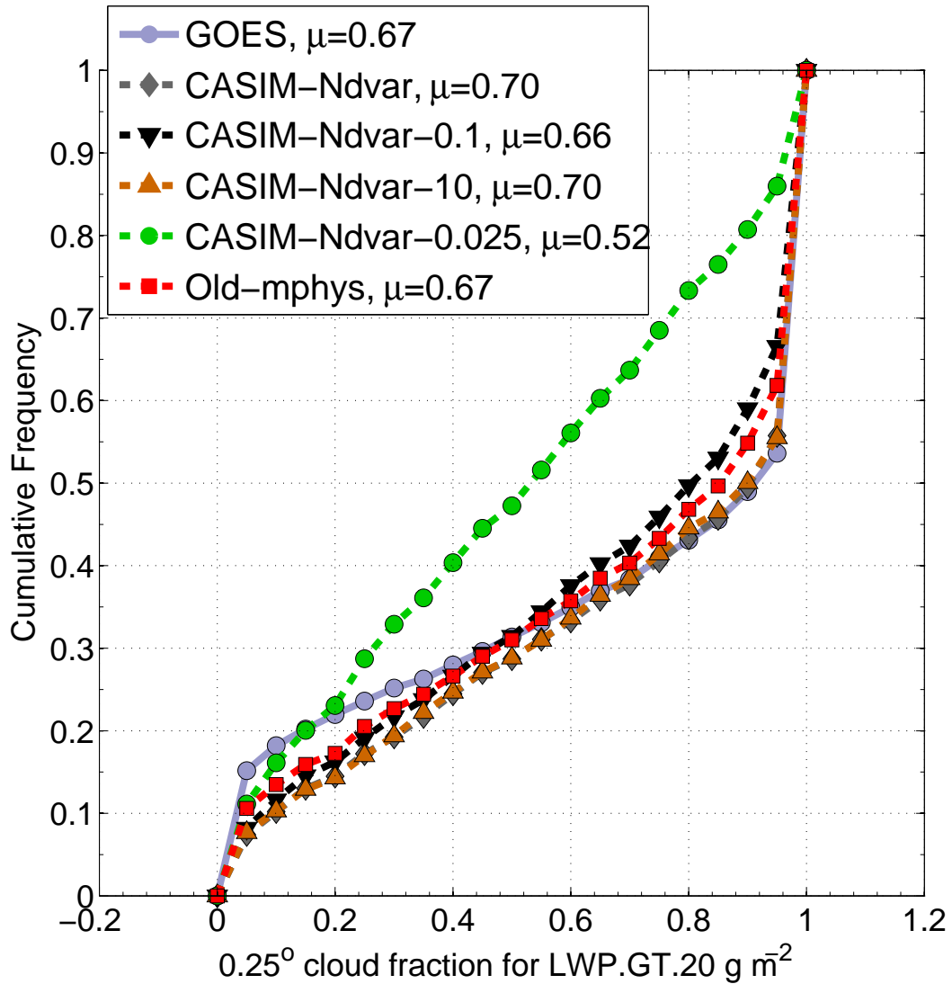
Figure 10. Cloud fraction cumulative distribution functions between 08:12 and 16:12 LST for the model and 07:57 and 15:57 for GOES-10 sampled every 30 minutes. Here each cloud fraction value is calculated as the fraction of datapoints with LWP greater than 20 \text{ gm}^{-2} relative to the total number of datapoints in 0.25^\circ \times 0.25^\circ areas. GOES-10 data is used at the native 4 km resolution and the model LWP data is first coarse grained to this resolution from the native 1 km resolution.
