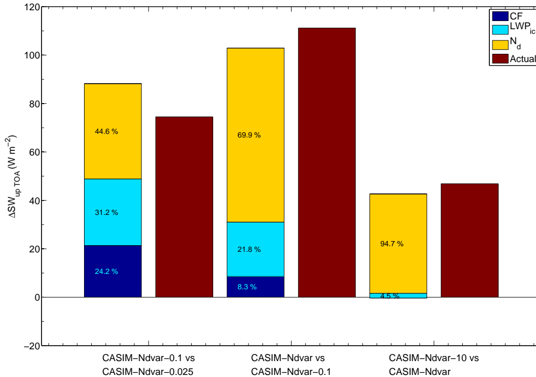
Figure 16. Estimated individual contributions to changes in the shortwave upwelling TOA radiation flux ( \Delta SW_{upTOA} ) due to changes in the domain and time mean (weighted as for Fig. 15) cloud properties (cloud fraction, f_c , in-cloud LWP, LWP_{ic} , and droplet number concentration, N_d , see the legend for the colour labelling) using an analytical formula for scene albedo. Changes in SW_{upTOA} are estimated between a given run in Fig. 15 ( Run_i ) and the run with the next highest aerosol concentration ( Run_{i+1} ) by replacing one cloud property of Run_i with that from Run_{i+1} ; i.e. for the f_c response, \Delta SW_{f_c} = SW(f_{c_{i+1}}, LWP_{ic_i}, N_{d_i}) - SW(f_{c_i}, LWP_{ic_i}, N_{d_i}) with the runs being compared indicated by the x-axis labels. The percentage that each cloud property contributes to the sum of the absolute changes is shown in the individual bars, e.g. the cloud fraction percentages are given by 100 \times \Delta SW_{f_c} / (|\Delta SW_{f_c}| + |\Delta SW_{LWP_{ic}}| + |\Delta SW_{N_d}|) . The red bars show the actual change in SW from the model output.
