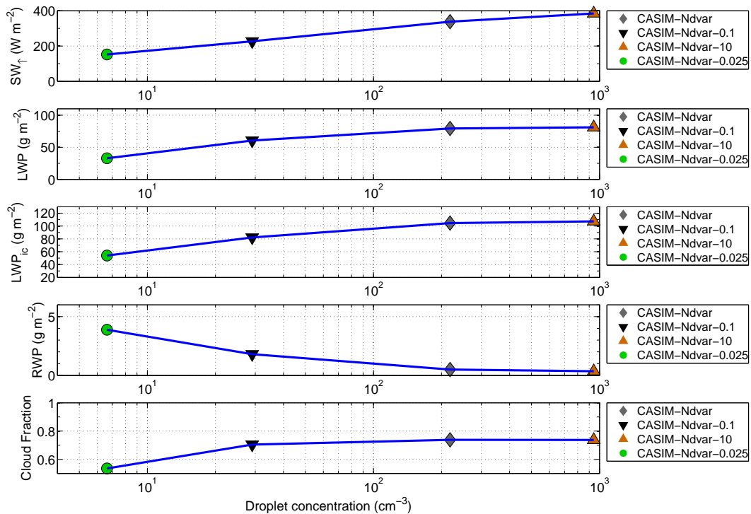
Figure 15. Summary plots of domain and time mean quantities for the different model runs. The time average is weighted by the incoming SW TOA flux timeseries to give extra weighting to times when the cloud properties will be contributing to the SW flux, i.e. mainly in the daytime. The x-axis shows droplet concentrations, which are calculated in the same way as for Fig 3. The top plot shows SW TOA flux, which is followed by LWP (domain mean), in-cloud LWP ( LWP_{ic} ), RWP and cloud fraction. Cloud fraction is calculated as for Fig. 10. Model data at 30 min intervals between the times of 06 UTC (01:12 LST) on 12th Nov and 0 UTC (19:12 LST) on 14th Nov are used, with the first six hours of model data being avoided due to spin-up.
