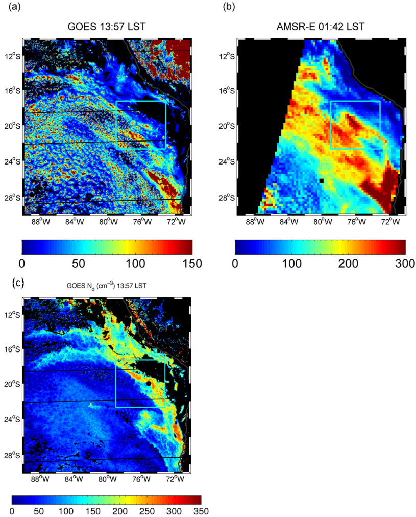
Figure 2. Snapshots of LWP (a and b, \text{gm}^{-2} ) and N_d (c) for 13th Nov, 2008. (a) and (c) 13:57 LST (daytime, 18:45 UTC) from the GOES-10 geostationary satellite at 4 km resolution. (b) 01:42 LST (nighttime, 06:30 UTC) from the AMSR-E instrument that has a lower resolution of 0.25^\circ (GOES-10 LWP and N_d retrievals are probably not reliable at nighttime). Note the different colour scales. The AMSR-E image has a region missing to the west due to the polar orbiting nature of the satellite and the limited swath width. Black regions in the LWP plots denote those where \text{LWP} < 20 \text{ gm}^{-2} , which we have chosen to define as cloud-free. The blue box shows the location of the 1 km resolution model domain.
