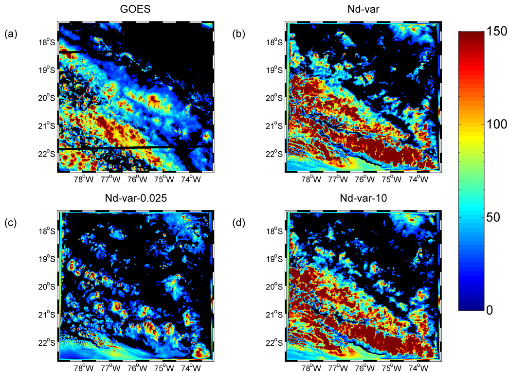
Figure 6. Daytime snapshots of LWP ( \text{gm}^{-2} ) for 13th Nov, 2008 for the region of the inner model domain. (a) GOES-10 satellite at 13:57 LST (daytime); (b) model with control aerosol; (c) model with x0.025 aerosol; (d) model with x10 aerosol. The model images are from 14:12 LST. Regions where the LWP is less than 20 \text{ gm}^{-2} are plotted as black to give an estimate of cloud fraction.
