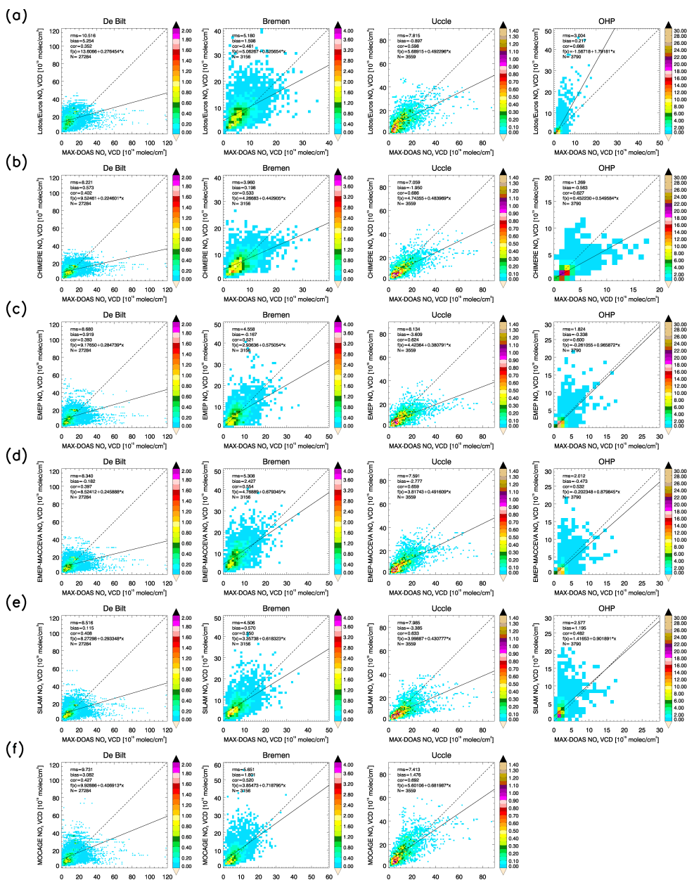
Figure A2. Scatter density plots of AVK-weighted tropospheric NO 2 VCDs [10 15 molec cm -2 ] from MAX-DOAS against model data for (from left to right) De Bilt, Bremen, Uccle and OHP. The data is shown for different bins with a size of 10 15 molec cm -2 and is colored according to the number of data points per bin [%]. The different panels show different model runs: (a) LOTOS-EUROS, (b) CHIMERE, (c) EMEP, (d) EMEP-MACCEVA, (e) SILAM and (f) MOCAGE. MOCAGE data is not available for the measurement time period at OHP. The dashed line is the reference line (f(x)=x). The solid line is the regression line (see top left of each plot for f(x) of this line). The root mean squared error (rms) [10 15 molec cm -2 ], bias [10 15 molec cm -2 ], Pearson correlation coefficient (cor, not squared) as well as the number of data points N are given at the top left of each plot.
