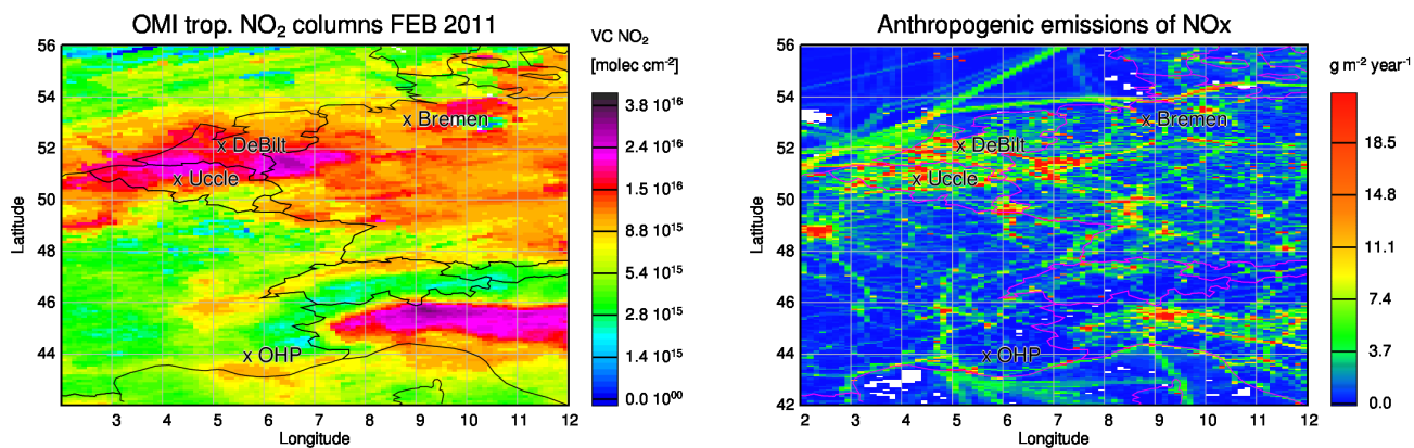
Figure 1. Maps of (left) average tropospheric NO 2 VCDs [molec cm -2 ] observed by OMI for February 2011 and (right) TNO/MACC-II anthropogenic NO x emissions [g m -2 year -1 ] over Europe. The location of MAX-DOAS measurement sites investigated in this study are marked by black crosses on the maps. The satellite data has been gridded to 0.1° lat x 0.1° lon, the resolution of the emission database is 0.125° lat x 0.0625° lon.
