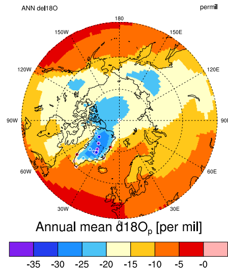
Figure 10. Annual mean \delta^{18}O_p for the CTRL run compared to observations
