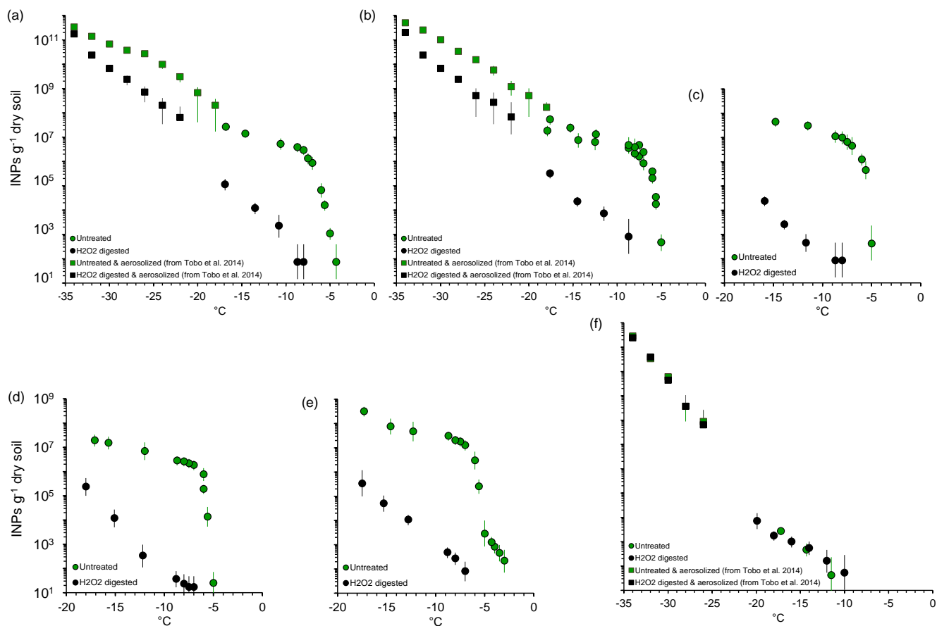
Fig. 2. Effect of removal of SOM by H_2O_2 digestion upon INP concentrations of soils. Soils are (a) sugar beet, (b) organic grass/alfalfa fallow, (c) pasture, (d) sagebrush shrubland, (e) lodgepole pine forest, and (f) kaolinite. The sugar beet, organic grass/alfalfa and kaolinite figures include data of aerosolized soil dusts ( 0.6 \mu m dia.) from Tobo et al., (2014) measured using a continuous flow diffusion chamber.
