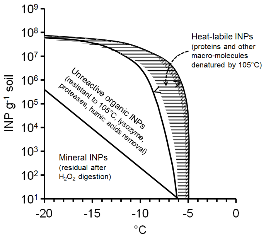
Fig. 12. Sources of ice nucleating particles in the pasture soil. Within the heat-labile segment, horizontal lines indicate IN proteins digested by papain (eg. from Mortierella alpina ), and diagonal lines INPs in live bacteria (sensitive to lysis with lysozyme). -The mineral INPs wedge is inherently approximate since \text{H}_2\text{O}_2 oxidation may not remove all SOM and cannot be assumed not to deactivate IN sites on some minerals.
