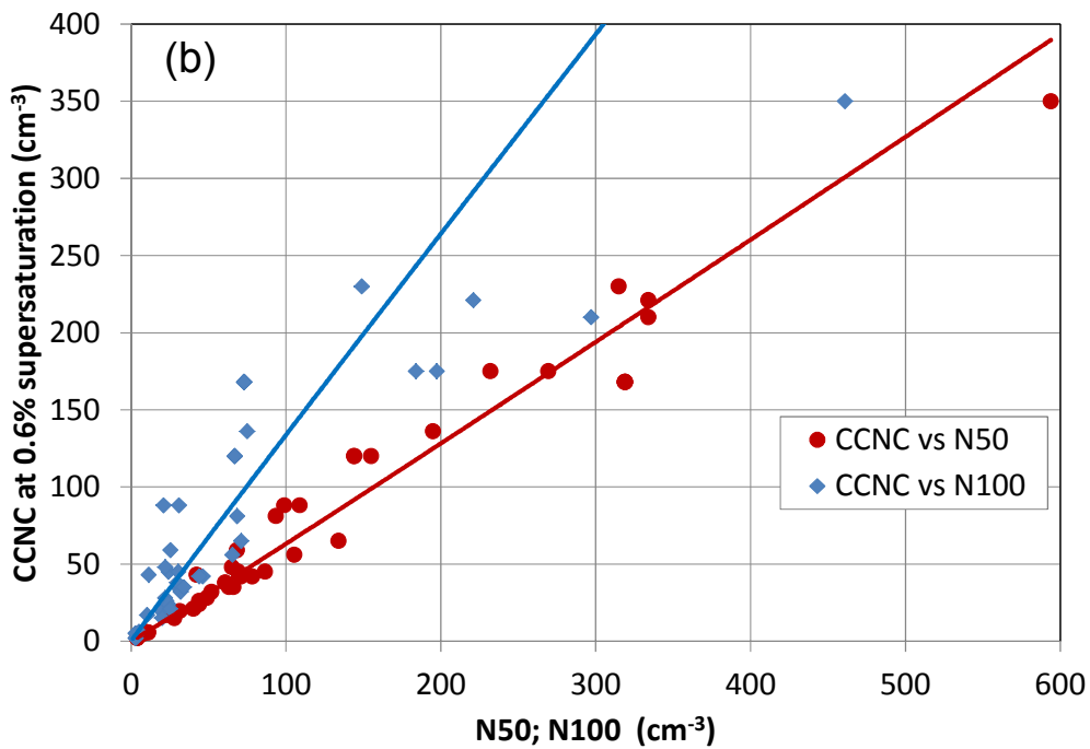
Figure 10. a) CDNC plotted versus the CCNC measured at 0.6% supersaturation; points are identified between LA (yellow) and HA (blue) samples, and linear regressions through the origin are shown; the CCNC(0.6%) points are limited to 44 of the 62 total, due to problems with the CCN measurement; the 44 are split 16 and 28 between LA and HA,. b) CCNC(0.6%) (44 points) plotted versus N50 and N100; power law fits to each are provided for reference.
