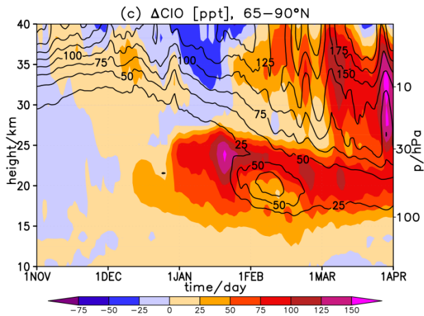
Figure 910. Colours: Time-altitude cross-sections of the Arctic mean differences between the years 2063 and 2060 in (a) ozone mixing ratios [ppm], (b) ozone number density [ 10^{12} molecules \text{cm}^{-3} ] and (c) ClO mixing ratio [ppt]. The solid contours show the year 2060 for reference.
