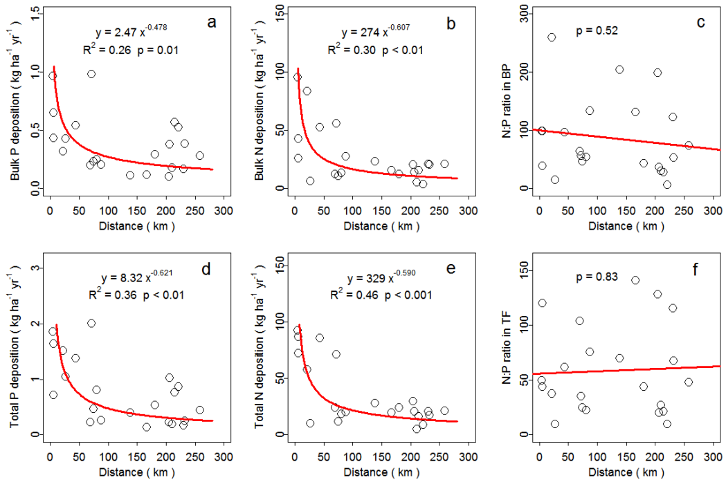
Figure 4. Changes in bulk deposition of P and N ( \text{kg ha}^{-1} \text{ yr}^{-1} ), total deposition of P and N ( \text{kg ha}^{-1} \text{ yr}^{-1} ), and N:P ratios in 5 bulk precipitation (BP) and throughfall (TF) with the distance to the nearest large cities based on datasets of forested sites far from semiarid regions in China.
