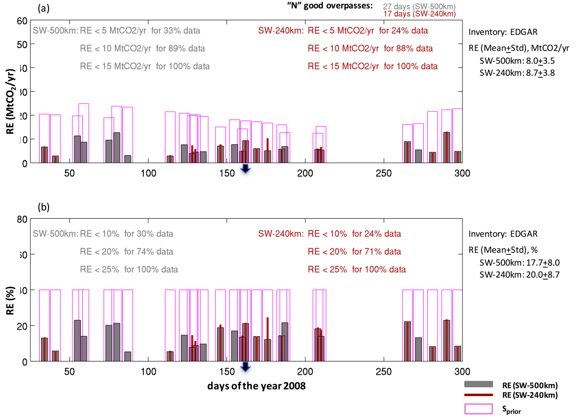
Figure 6: Precision (random errors (RE)) of the retrieved emission fluxes obtained by the inverse optimization using one year of CarbonSat simulated observations. Results of two different swath widths (SW) – 500 km (grey) and 240 km (red) – are shown. S_{prior} values are indicated with magenta bordered bars for visualizing the reduction in uncertainty. The top and bottom panels show RE in MtCO 2 yr -1 and in % respectively. An overview of the statistical distribution of RE, separately for 500 km (grey) and 240 km (red) swath widths, is given inside the panel. The overall mean ± standard deviation is given outside the respective panels. The lower and upper limits of the X-axis (days of the year) is restricted accordingly as there are no good CarbonSat simulated observation during winter months. The arrow marker in the X-axis indicates a particular day (24 th June 2008) shown in Figs. 4, 7, and 8.
