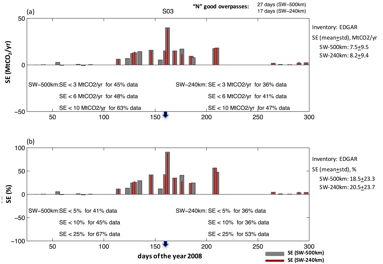
Figure 11: Same as Fig.9, but for S03, quantifying the impact of the worst-case modeling related errors by assuming that biogenic XCO 2 variations cannot be modeled at all.
