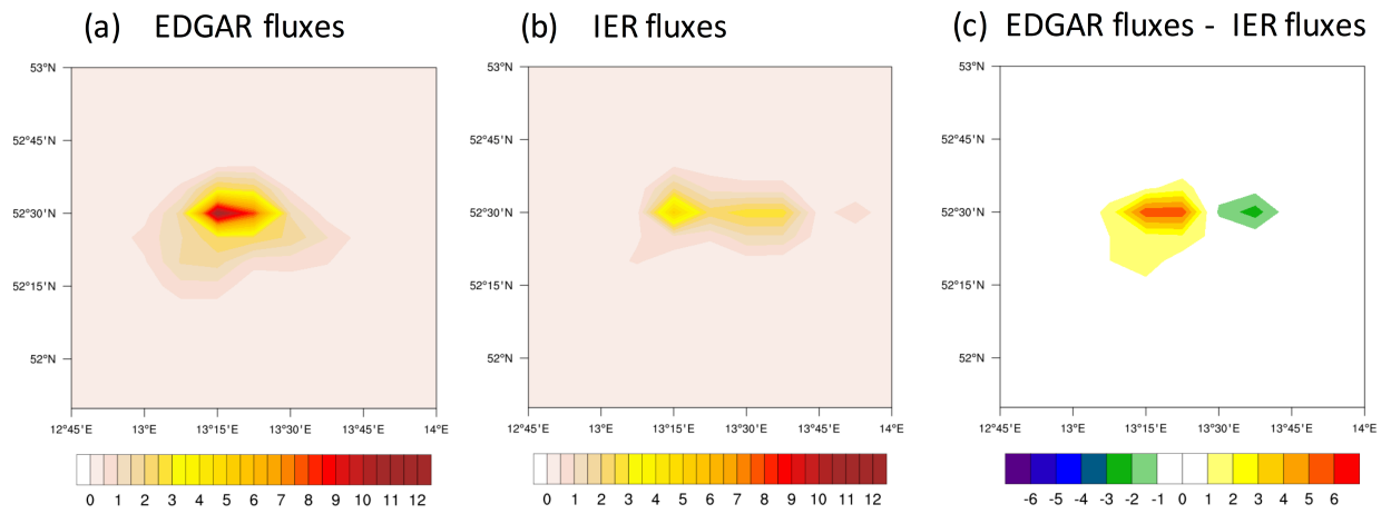
Figure 2: Annual averages of fossil fuel combustion emission fluxes at 10 \text{ km} \times 10 \text{ km} , zoomed over the Berlin region: (a) EDGAR emissions, (b) IER emissions, and (c) the difference between EDGAR and IER emissions (EDGAR - IER). All units are in \text{MtCO}_2 per year per grid cell.
