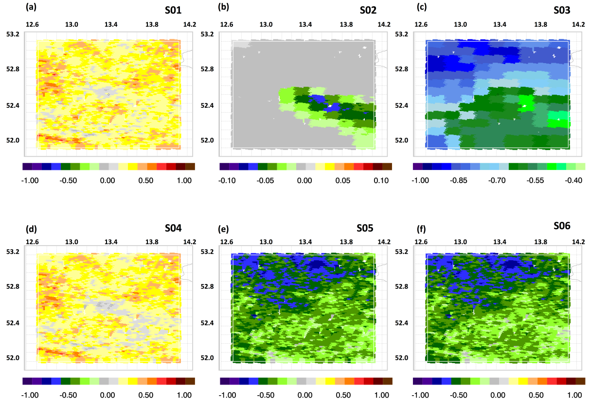
Figure 7: XCO 2 systematic error over the target region on 24 th June 2008, assuming a CarbonSat swath width of 500 km. The six scenarios (S01 to S06) are shown with a label inside the respective panel. For S01, S02 and S04, these errors are estimated using the error parameterization scheme of Buchwitz et al. (2013a). The other scenarios additionally utilize biogenic XCO 2 variability in the target region (simulated by WRF-GHG) to derive XCO 2 systematic errors. Note that different color scales are used for S02 and S03. All units are given in ppm.
