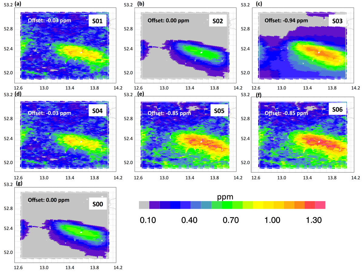
Figure 8: Observed anthropogenic XCO 2 enhancement over the target region during a CarbonSat overpass on 24 th June 2008 (swath width: 500 km). Different panels show anthropogenic XCO 2 enhancement, while considering XCO 2 systematic errors for different scenarios as shown in Fig.8. The “True” XCO 2 (fossil fuel (FF)) enhancement (i.e. without any uncertainties) is given in the bottom panel (g) for comparison. Note that an offset, labeled inside each panel, is subtracted from the anthropogenic XCO 2 enhancement to better visualize the details (for the figure only). All units are ppm.
