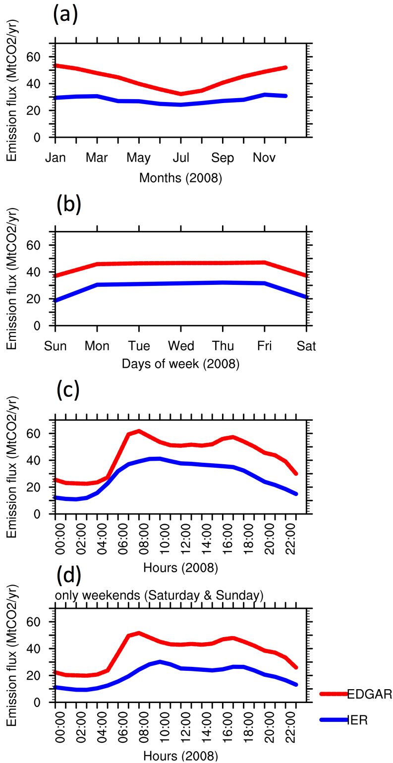
Figure 3: Temporal variability of EDGAR and IER emission fluxes, aggregated over the target region around Berlin (~100 km × 100 km) averaged for different time scales for the year 2008: (a) monthly, (b) weekly and (c & d) hourly. The 4 th panel (d) shows the values representing only weekends, while the 3 rd panel (c) represents all days of the week. Hours are in UTC (local time CET = UTC+1).
