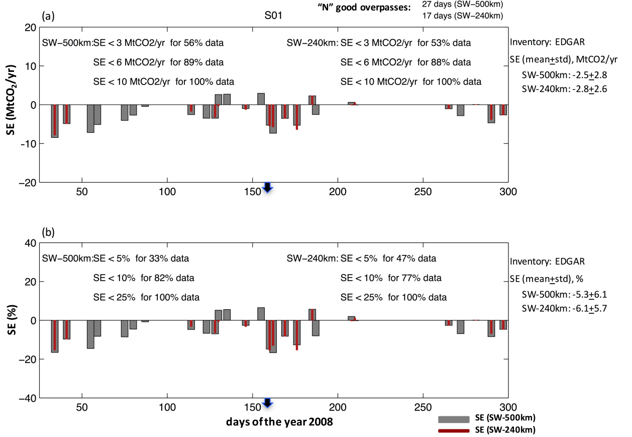
Figure 9: Systematic errors (SE) of the retrieved emission fluxes for S01, obtained by the inverse optimization using one year of CarbonSat simulated observations. Results of two different swath widths (SW) – 500 km (grey) and 240 km (red) – are shown. (a) and (b) show SE in MtCO 2 yr -1 and in % respectively. An overview of the statistical distribution of SE, separately for 500 km (grey) and 240 km (red) swath widths, is given inside the panel. The overall mean +/- standard deviation is given outside the respective panels.
