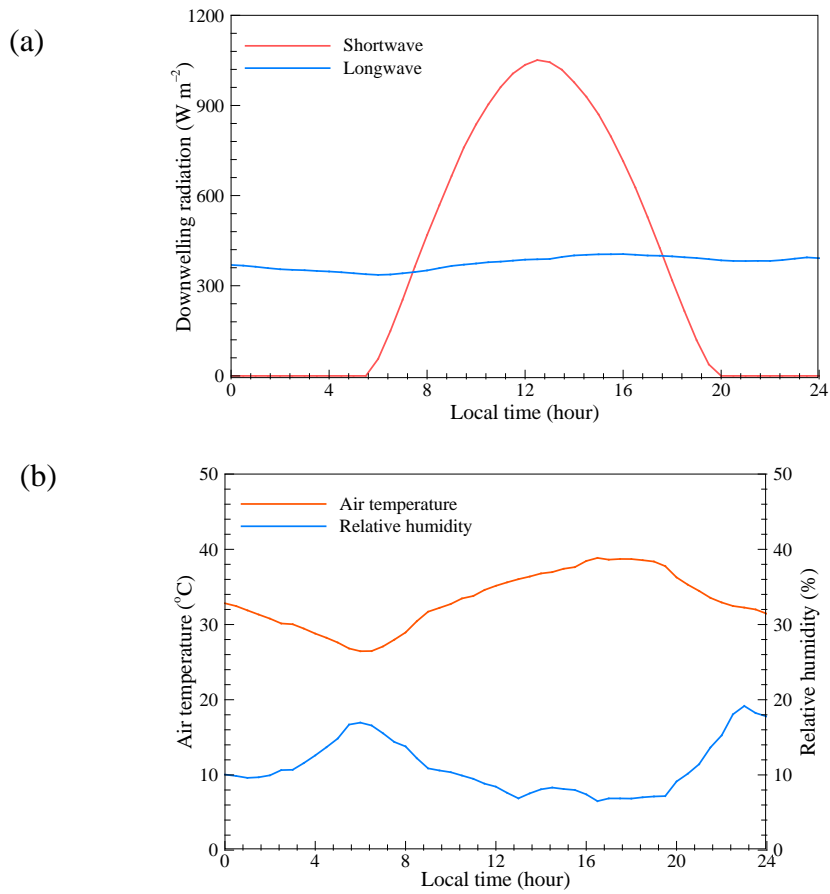
Figure 5: The diurnal surface atmospheric forcing of June 14, 2012 (a clear day) in Phoenix, AZ: (a) downwelling shortwave and longwave radiation and (b) air temperature and relative humidity. The daytime data between starting point (6:00 am local time) and ending point (7:30 pm local time) are used to drive the SLUCM-SCM under convective condition.
