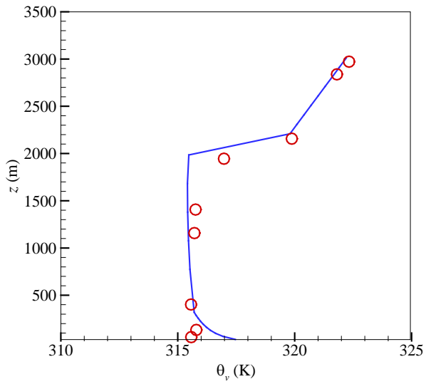
Figure 2: Comparison of simulated and measured atmospheric profiles of virtual potential temperature \theta_v and specific humidity q for two time points, i.e. (a) 16:44 pm (local time) on July 2 nd , 2013, and (b) 16:37 pm (local time) on July 9 th , 2013 at NOAA-ESRL Phoenix site.
