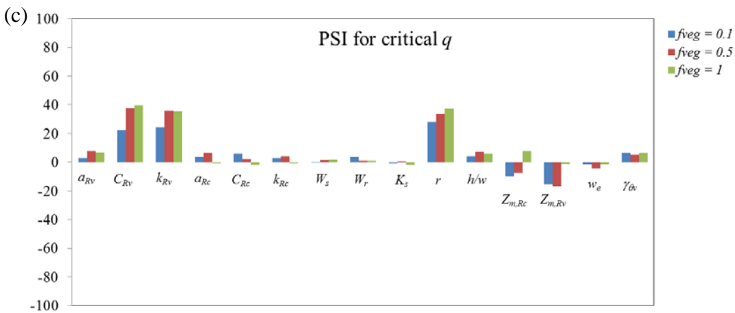
Figure 8: PSI values for model outputs of critical (a) z_h , (b) mixed layer \theta_v , and (c) mixed layer q , with different green roof fractions.
