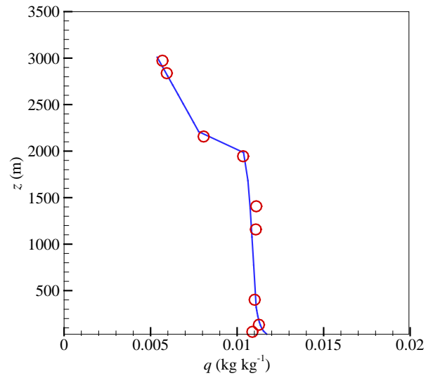
Figure 2: Comparison of simulated and measured atmospheric profiles of virtual potential temperature \theta_v and specific humidity q for two time points, i.e. (a) 16:44 pm (local time) on July 2 nd , 2013, and (b) 16:37 pm (local time) on July 9 th , 2013 at NOAA-ESRL Phoenix site.
