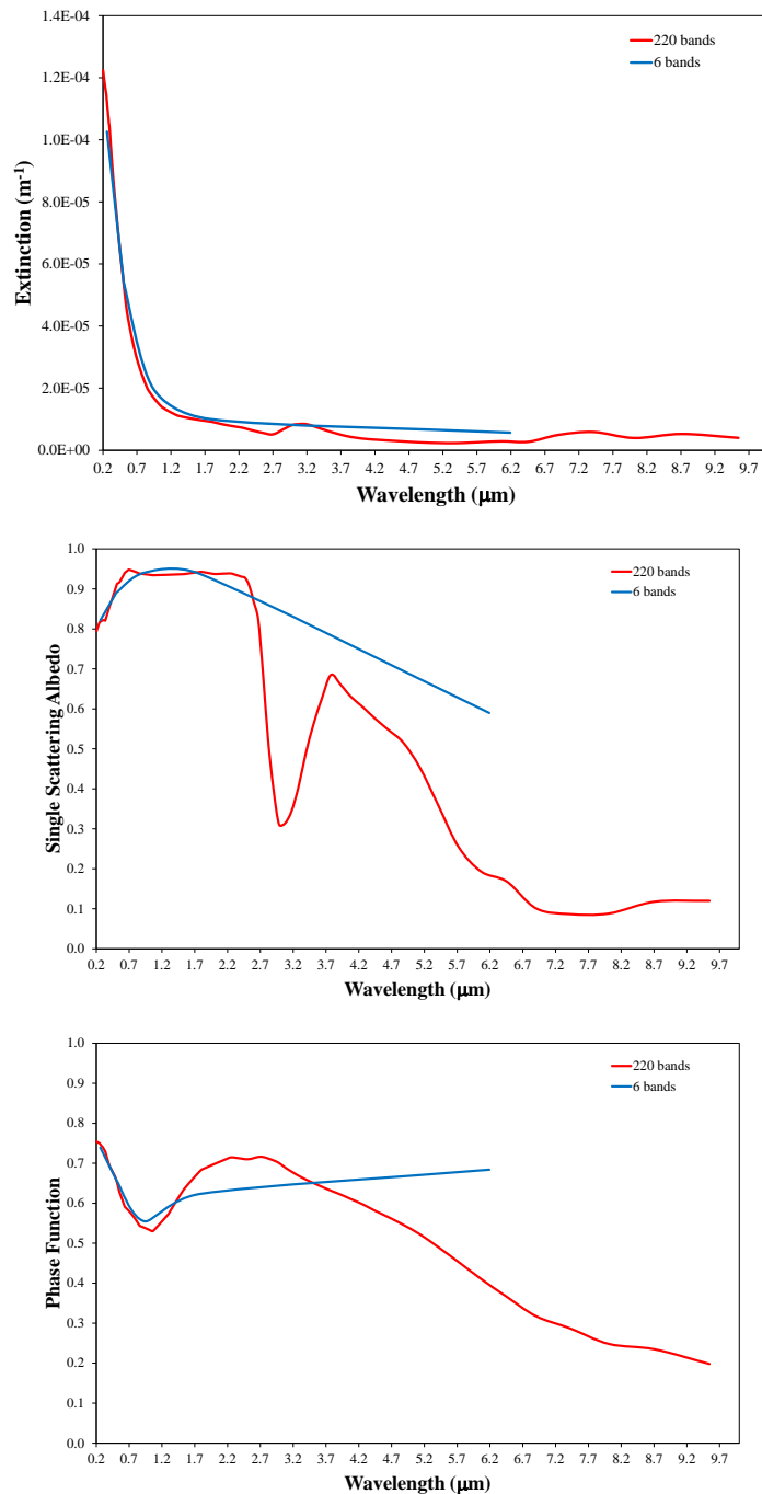
Fig. S1. Spectral dependence of the aerosol extinction (top), the single scattering albedo (middle) and the phase function (bottom) over the range 0.2 - 10 μm.
