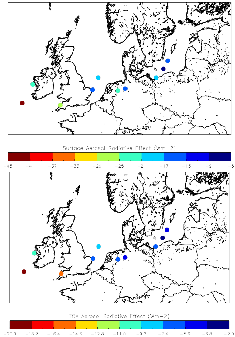
Figure 3. Aerosol radiative effect in Wm -2 at the surface (top) and TOA (bottom) across north-western Europe during EUCAARI-LONGREX.
