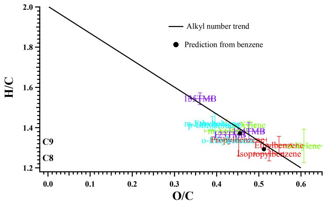
Fig. 3. H/C vs. O/C in SOA formed from different aromatic hydrocarbon photooxidation under low NO x colored by aromatic isomer type and marked with individual aromatic hydrocarbon species (C8 and C9 on the lower left indicate the location of initial aromatic hydrocarbon precursor): Ethylbenzene 2084A; Propylbenzene 1245A; Isopropylbenzene 1247A; m -Xylene 1191A; m -Ethyltoluene 1199A; o -Xylene 1320A; o -Ethyltoluene 1179A; p -Xylene 1308A; p -Ethyltoluene 1194A; 1, 2, 3-Trimethylbenzene (123TMB) 1162A; 1, 2, 4-Trimethylbenzene(124TMB) 1119A; 1, 3, 5-Trimethylbenzene(135TMB) 1156A. Alkyl number trend is the linear fitting in (Li., et al., 2015a). Solid black cycles are SOA elemental ratio from C 8 and C 9 aromatic hydrocarbon predicted by SOA elemental ratio formed from benzene. *Error bar stands for H/C and O/C standard deviation when significant particles are formed (>5μg/m 3 ).
