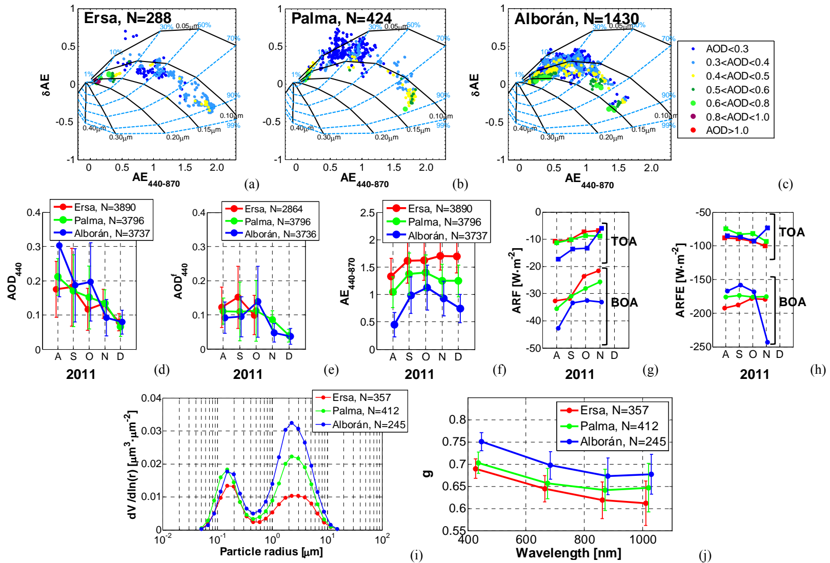
Figure 13. ( \delta AE , AE ) plot at (a) Ersa, (b) Palma and (c) Alborán over the whole period; monthly variations of (d) aerosol optical depth at 440 nm ( AOD_{440} ), (e) the fine mode aerosol optical depth at 440 nm ( AOD_{440}^f ), (f) the Ångström exponent AE_{440-870} , (g) the aerosol radiative forcing (ARF) and (h) the aerosol radiative forcing efficiency (ARFE); (i) the columnar size distribution and (j) spectra of the asymmetry factor ( g ) averaged over the whole period. The data are from AERONET level 2.0 inversion products during the period August to December 2011. BOA and TOA stand for bottom and top of the atmosphere, respectively. The numbers of points in the plots (g) and (h) (not indicated in the plots for the sake of clarity) are 123, 133 and 101 for Ersa, Palma and Alborán, respectively. The color code is the same in all figures (d)-(j): red, green and blue for Ersa, Palma and Alborán, respectively. In (g)-(h) the error bars have been omitted for the sake of clarity.
