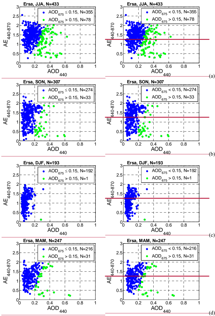
5 Figure 2. Ångström exponent calculated between 440 and 870 nm ( AE_{440-870} ) as a function of the aerosol optical depth at 440 nm ( AOD_{440} ) at Ersa during (a) summer, (b) autumn, (c) winter and (d) spring, for the whole 2011-2015 AERONET level 2.0 daily AOD dataset. Blue bullets are for AOD_{675} < 0.15 and green bullets for AOD_{675} > 0.15
