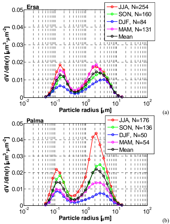
Figure 7. Seasonal variation of the particle volume size distribution in the atmospheric column at (a) Ersa and (b) Palma derived from AERONET level 2.0 daily inversion products available in the period 2011 – 2015.
