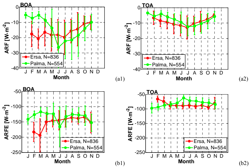
Figure 12. Monthly variation of (a) the solar aerosol radiative forcing (ARF) and of (b) the solar aerosol radiative forcing efficiency (ARFE) at the (1) bottom of the atmosphere (BOA) and (2) at the top of the atmosphere (TOA), derived from AERONET level 2.0 inversion products available in the period 2011-2015. Both the ARF and the ARFE were estimated for 50 \leq \text{Solar Zenith Angle (SZA)} \leq 60^\circ . The error bars represent the standard deviation.
