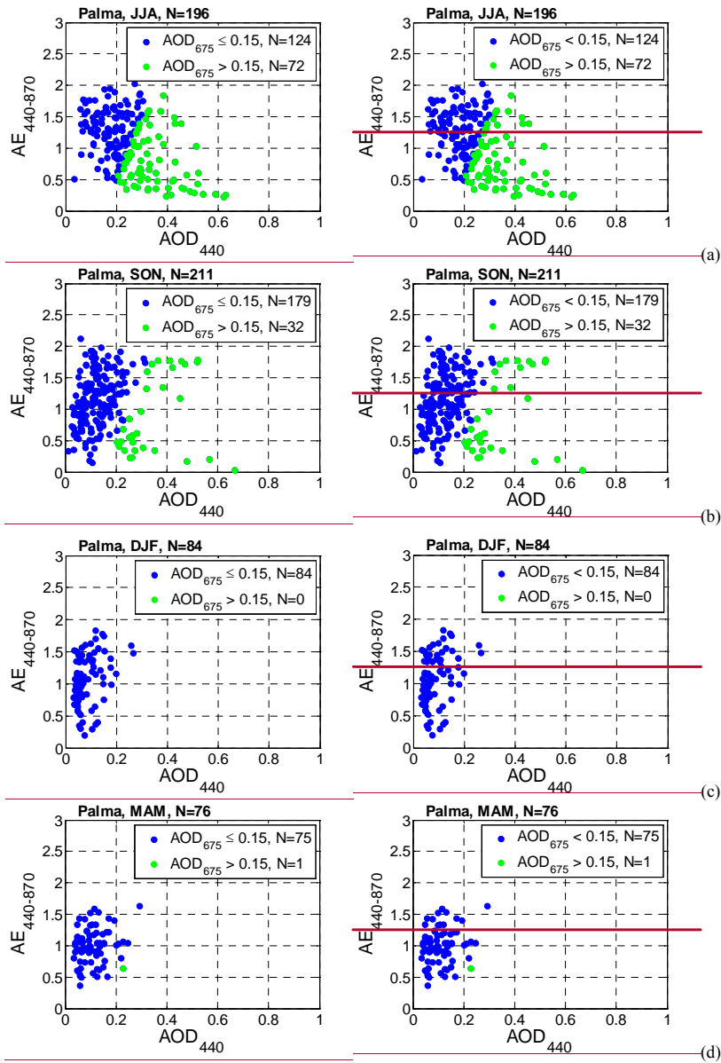
5 Figure 3. Ångström exponent calculated between 440 and 870 nm ( AE_{440-870} ) as a function of the aerosol optical depth at 440 nm ( AOD_{440} ) at Palma during (a) summer, (b) autumn, (c) winter and (d) spring, for the whole 2011-2015 AERONET level 2.0 daily AOD dataset. Blue bullets are for AOD_{675} \leq 0.15 and green bullets for AOD_{675} > 0.15 .
