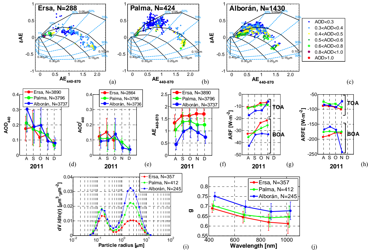
Figure 13. ( \delta AE, AE) plot at (a) Ersa, (b) Palma and (c) Alborán over the whole period from August to December 2011 ; monthly variations of (d) aerosol optical depth at 440 nm (AOD 440 ), (e) the fine mode aerosol optical depth at 440 nm ( AOD'_{440} ), (f) the Ångström exponent AE_{440-870} , (g) the aerosol radiative forcing (ARF) and (h) the aerosol radiative forcing efficiency (ARFE); (i) the columnar size distribution and (j) spectra of the asymmetry factor (g) averaged over the whole period. The data are from AERONET level 2.0 inversion products during the period August to December 2011. BOA and TOA stand for bottom and top of the atmosphere, respectively. The numbers of points in the plots (g) and (h) (not indicated in the plots for the sake of clarity) are 123, 133 and 101 for Ersa, Palma and Alborán, respectively. The color code is the same in all figures (d)-(j): red, green and blue for Ersa, Palma and Alborán, respectively. In (g)-(h) the error bars have been omitted for the sake of clarity.
