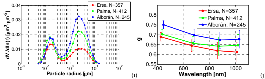
Figure 1344. ( \delta AE, AE) plot at (a) Ersá, (b) Palma and (c) Alborán over the whole period; monthly variations of (d) aerosol optical depth at 440 nm ( AOD_{440} ), (e) the fine mode aerosol optical depth at 440 nm ( -AOD_{440}^f ), (f) the Ångström exponent AE_{440-870} , (g) the aerosol radiative forcing (ARF) and (h) the aerosol radiative forcing efficiency (ARFE); (i) the columnar size distribution and (j) spectra of the asymmetry factor ( -g ) averaged over the whole period. The data are from AERONET level 2.0 inversion products during the period August to December 2011. BOA and TOA stand for bottom and top of the atmosphere, respectively. The numbers of points in the plots (g) and (h) (not indicated in the plots for the sake of clarity) are 123, 133 and 101 for Ersá, Palma and Alborán, respectively. The color code is the same in all figures (d)-(j): red, green and blue for Ersá, Palma and Alborán, respectively. In (g)-(h) the error bars have been omitted for the sake of clarity.
