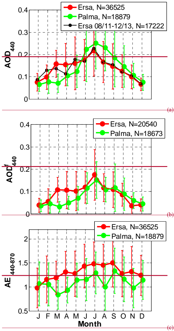
Figure 64. Monthly average variations calculated with instantaneous-daily measurements of a) aerosol optical depth at 440 nm ( AOD_{440} ) ; b) fine mode aerosol optical depth at 440 nm ( AOD_{440}^f ) ; and c) the Ångström exponent calculated between 440 and 870 nm ( AE_{440-870} ) derived from AERONET level 2.0 inversion products available in the period 2011 – 2015. The error bars represent the standard deviation. On the AOD_{440} plot we have also plotted the monthly values at Ersa calculated over the limited period for which data are also available at Palma, i.e. August 2011 – December 2013.
