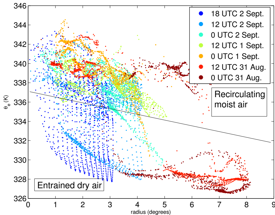
Figure 9. \theta_e and radial distance from the center of Gaston's pouch. The colors range from brown to blue, with brown denoting the earliest time of 00:00 UTC 31 August and blue denoting the latest time of 18:00 UTC 2 September.
