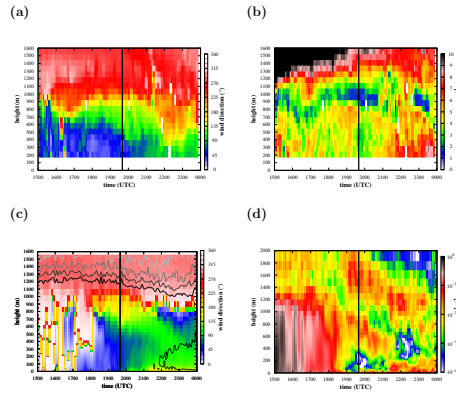
new Figure 4. Temporal evolution of the observed (UHF) and modelled vertical profiles for (a) UHF wind direction (in ^{\circ} ), (b) UHF wind speed (in \text{m s}^{-1} ), (c) MesoNH wind direction (in colours) and wind speed (in lines, for values \geq 4 \text{ m s}^{-1} , contour interval = 2 \text{ m s}^{-1} ) and (d) MesoNH TKE (in \text{m}^2 \text{ s}^{-2} ). The time of sunset is represented with a black vertical line.
