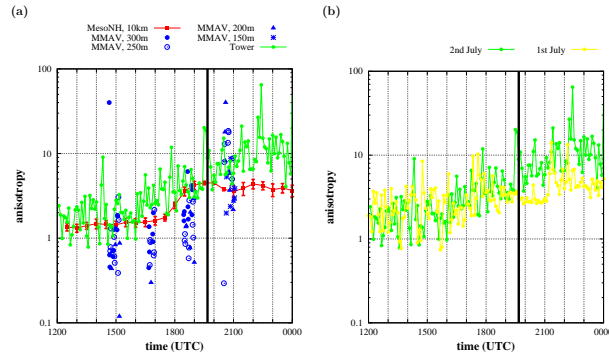
Figure 7. (a) Time series of the anisotropy computed from different sources: M^2 AV flight observations during the four flights for different heights (in blue); tower measurements at 60 m AGL every 5 min (in green); and model results averaged between 150 m and 300 m AGL to be close to the altitudes of the M^2 AV observations considering a spatial area of 10 km x 10 km centered at Lannemezan (in red). The time of sunset is represented with a black vertical line. Note the logarithmic scale on the y-axis.
