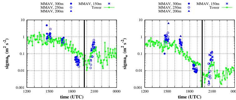
sigma-v and sigma-w separately computed from M 2 AV and the 60 m tower observations.
