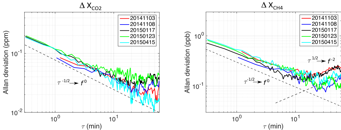
Figure 1. Allan deviation \sigma_{allan,\Delta X_{CO_2}} and \sigma_{allan,\Delta X_{CH_4}} as a function of the integrating time \tau . The black dashed lines represent a slope of -1/2 and a slope of 1/2 , which correspond to power spectral densities S(f) = f^0 (white noise) and S(f) = f^{-2} (Brownian noise), respectively. The Allan deviation follows a slope of -1/2 up to an integration time of 10 to 20 min, and then stays constant ( S(f) = f^{-1} ), and subsequently turns over to a slope of 1/2 , which describes a linear drift.
