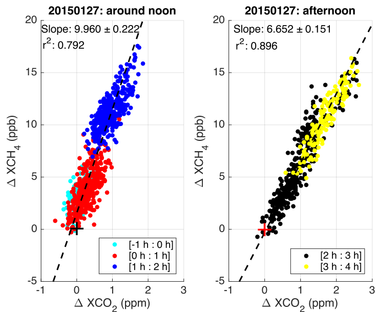
Figure 6. Column difference ratio measured across Pasadena colored by hours. Left figure shows the time period between 1 hour before solar noon and 2 hours after solar noon, and right figure shows the time period 2 to 4 hours after solar noon. The solar noon is about 12:05 local time. Both regression curves essentially pass through the origins that are shown as crosses.
