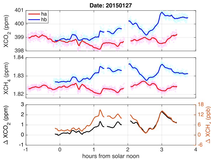
Figure 4. First and second panels: measured X_{\text{CO}_2} and X_{\text{CH}_4} north ( ha ) and south ( hb ) of Pasadena on 27 Jan. with 5 minutes averaging time. Third panel: \Delta X_{\text{CO}_2} and \Delta X_{\text{CH}_4} are temporally correlated and their ratio is determined as 7.8 ppb/ppm, shown in Fig. 5.
