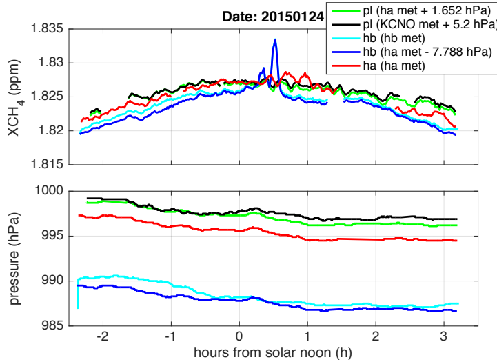
Figure 10. Surface pressure inputs (lower panel) and the corresponding X_{\text{CH}_4} retrieval results averaged for 5 min (upper panel). For Fig. 3(c) and the simple column model calculations, ha , hb and pl retrievals with the surface pressure inputs based on ha pressure measurements are used (red, blue and green curves).
