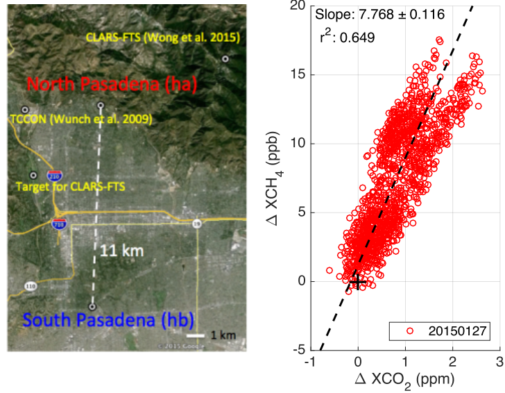
Figure 5. The derived ratio of column differences across Pasadena is consistent with Wunch et al. (2009) using TCCON DMF daily dynamics and very close to the excess ratio determined in Wong et al. (2015), which compared DMFs from diffuse solar reflectance off a spectralon plate at Mount Wilson with those from reflected sunlight from West Pasadena. Map provided by Google Earth, Image Landsat, Data SIO, NOAA, U.S. Navy, NGA, and GEBCO.
