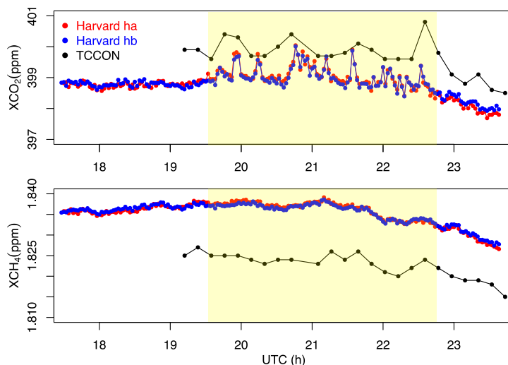
Figure 7. Side by side measurements on the roof of Caltech (17 Jan. 2015). Both EM27/SUN spectrometers (2 minutes block-average) captured short-term variations in the X_{\text{CO}_2} signal ( \sim 1 ppm corresponds to 0.25% relative). The TCCON spectrometer does not resolve these short-term variation due to the low measurement rate.
