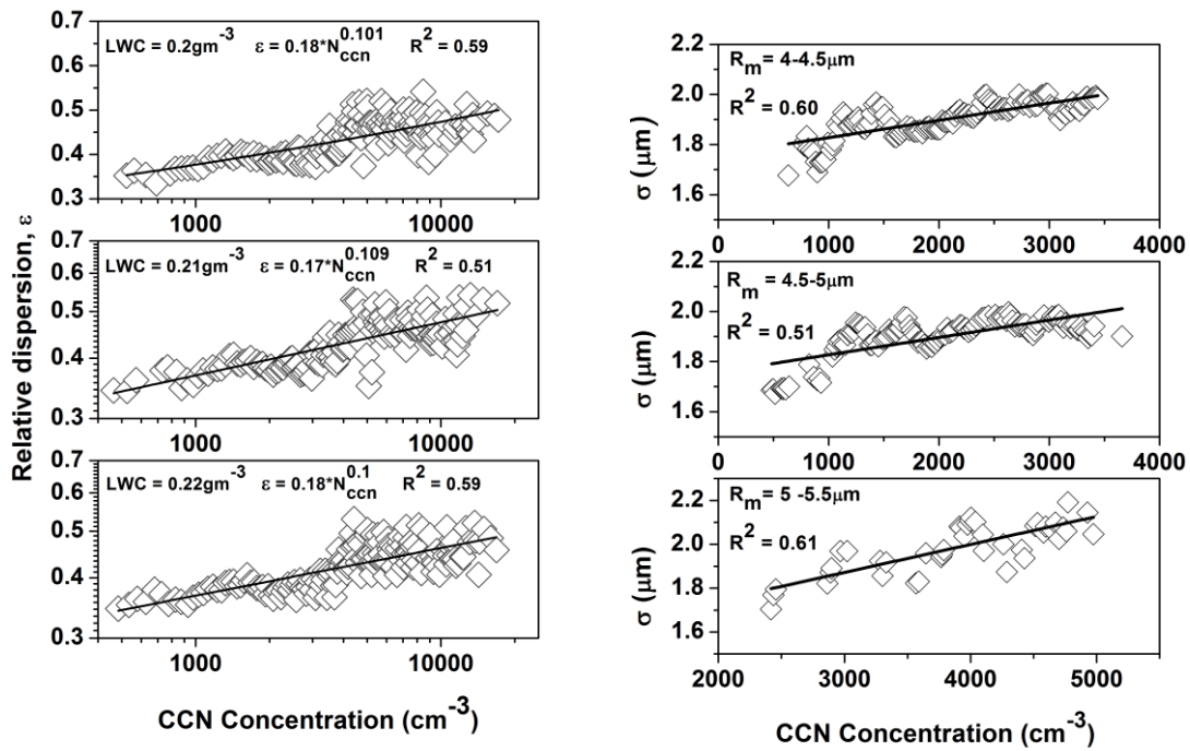
Figure 6a and 6b. Change in relative dispersion and spectral width of cloud droplet spectra with CCN concentration.
