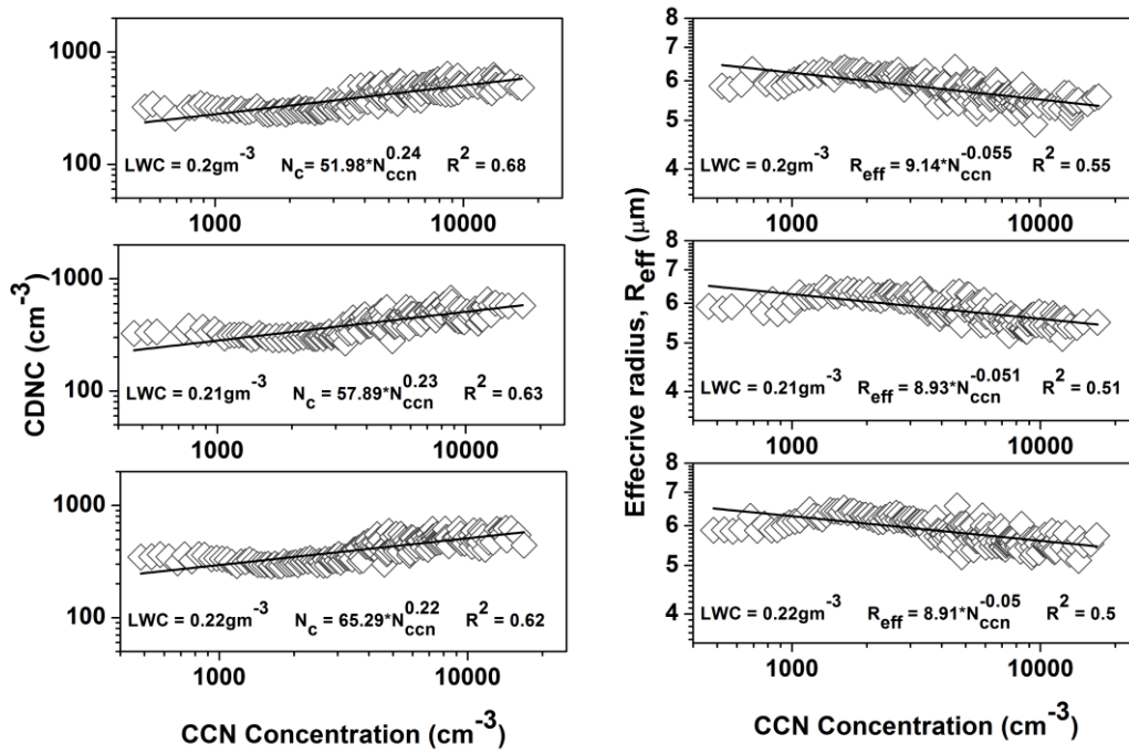
15 Figure 3 a and b. Variation of CDNC and effective radius with CCN concentration at 0.6% supersaturation for three LWC bins namely 0.20, 0.21 and 0.22 gm -3 .
