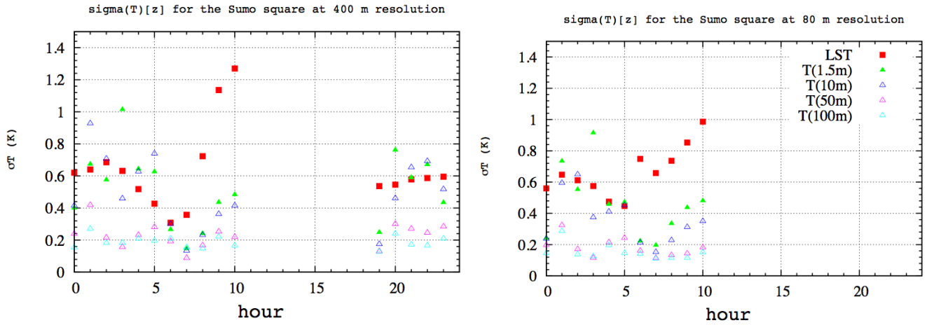
Figure 7. Evolution of the standard deviation of temperature in the SUMO square computed from D2 (left, run only between July 1 at 1800 UTC and July 2 at 1000 UTC) and from D3 (right, run only between 0000 and 1000 UTC of July 2)
