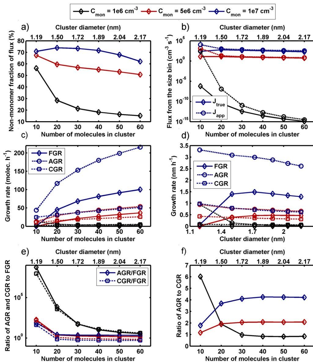
Figure 4. The effect of steady-state monomer concentration (shown as different colors) on quantities describing cluster growth in the presence of stable small clusters : a) non-monomer fraction of flux from each size bin, b) the true collision-evaporation flux from each size bin ( J_{\text{true}} ; solid line) and the fluxes calculated from the appearance times of clusters ( J_{\text{app}} ; dashed line), c) and d) flux-equivalent growth rate (FGR; solid line), growth rate derived from the appearance times of clusters (AGR; dashed line), and growth rate calculated based on irreversible vapor condensation (CGR; dotted line), e) the ratios of AGR to FGR (solid line) and CGR to FGR (dotted line), f) the ratio of AGR to CGR.
