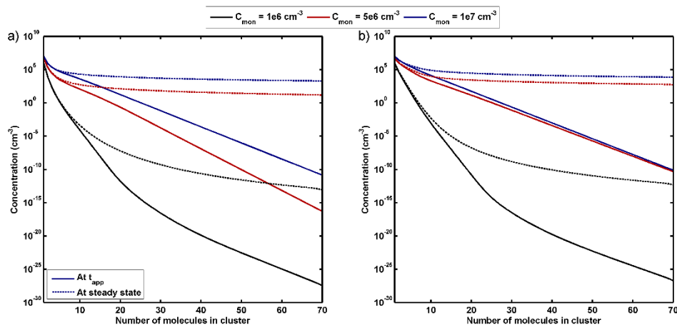
Figure A3. Cluster distribution at the mean appearance time of the two smallest size bins (solid lines) and at the final steady state (dashed lines) when a) the Gibbs free energy profile has one maximum and no minima b) the Gibbs free energy profile has an additional negative term corresponding to the stabilization of the smallest clusters. The colors show the steady state monomer concentration.
