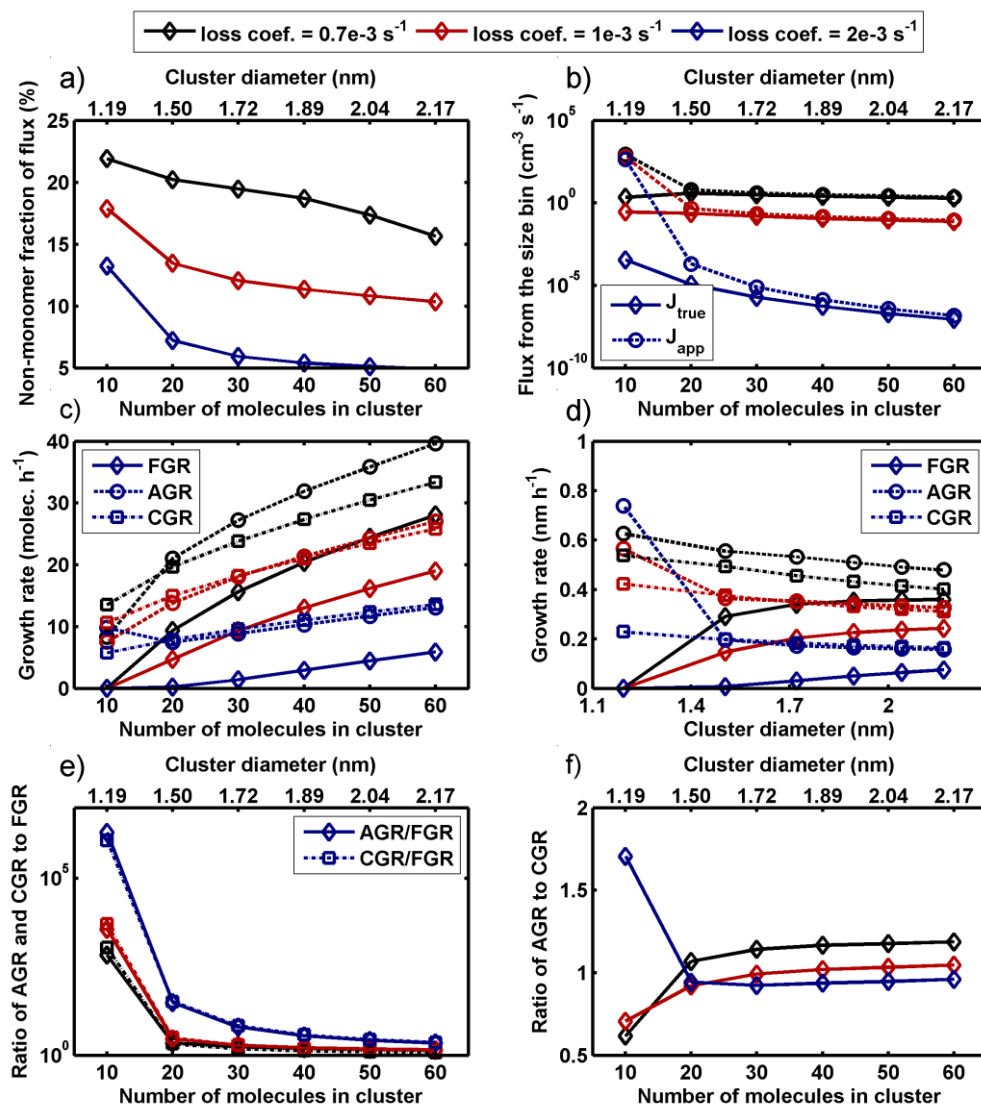
Figure A2. The effect of loss coefficient (shown as different colors) on quantities describing cluster growth in the presence small stable clusters: a) non-monomer fraction of flux from each size bin, b) collision- evaporation flux from each size bin ( J_{true} ; solid line) and the fluxes calculated from the appearance times of clusters ( J_{app} ; dashed line), c) and d) flux-equivalent 5 growth rate (FGR; solid line), growth rate derived from the appearance times of clusters (AGR; dashed line), and growth rate calculated based on irreversible vapor condensation (CGR; dotted line), e) the ratios of AGR to FGR (solid line) and CGR to FGR (dashed line), f) the ratio of AGR to CGR.
