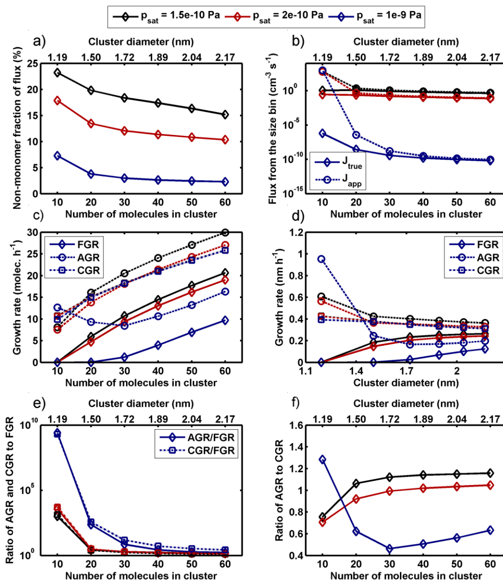
Figure 2. The effect of saturation vapor pressure (shown as different colors) on quantities describing cluster growth: a) non-monomer fraction of flux from each size bin, b) the true collision-evaporation flux from each size bin ( J_{\text{true}} ; solid line) and the fluxes calculated from the appearance times of clusters ( J_{\text{app}} ; dashed line), c) and d) flux-equivalent growth rate (FGR; solid line), growth rate derived from the appearance times of clusters (AGR; dashed line), and growth rate calculated based on irreversible vapor condensation (CGR; dotted line), e) the ratios of AGR to FGR (solid line) and CGR to FGR (dotted line), f) the ratio of AGR to CGR.
