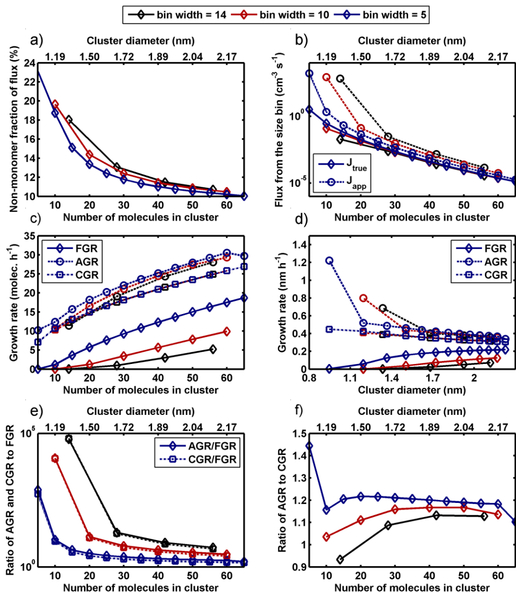
Figure 3. The effect of size bin width (shown as different colors) on quantities describing cluster growth: a) non-monomer fraction of flux from each size bin, b) the true collision-evaporation flux from each size bin ( J_{\text{true}} ; solid line) and the fluxes calculated from the appearance times of clusters ( J_{\text{app}} ; dashed line), c) and d) flux-equivalent growth rate (FGR; solid line), growth rate derived from the appearance times of clusters (AGR; dashed line), and growth rate calculated based on irreversible vapor condensation (CGR; dotted line), e) the ratios of AGR to FGR (solid line) and CGR to FGR (dotted line), f) the ratio of AGR to CGR.
