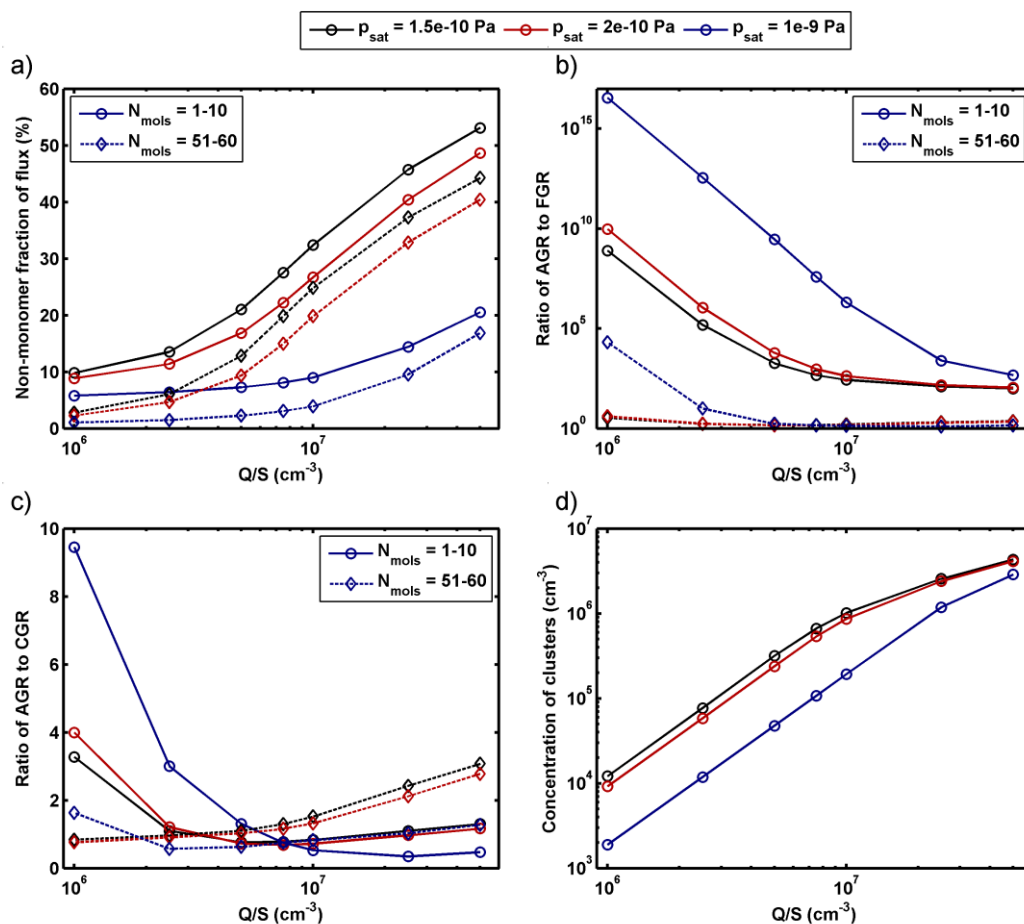
Figure 5. The results of the simulations with different saturation vapor pressures ( p_{sat} ; shown as different colors) and different ratios of monomer source rate to the loss coefficient ( Q/S ; shown on the x -axis) in the smallest size bin (solid line) and in the largest size bin (dashed line): a) non-monomer fraction of the flux, b) the ratio of appearance time growth rate (AGR) to flux-equivalent growth rate (FGR), c) the ratio of appearance time growth rate to growth rate calculated based on irreversible vapor condensation (CGR), d) steady state concentration of all clusters (2–70-mers).
