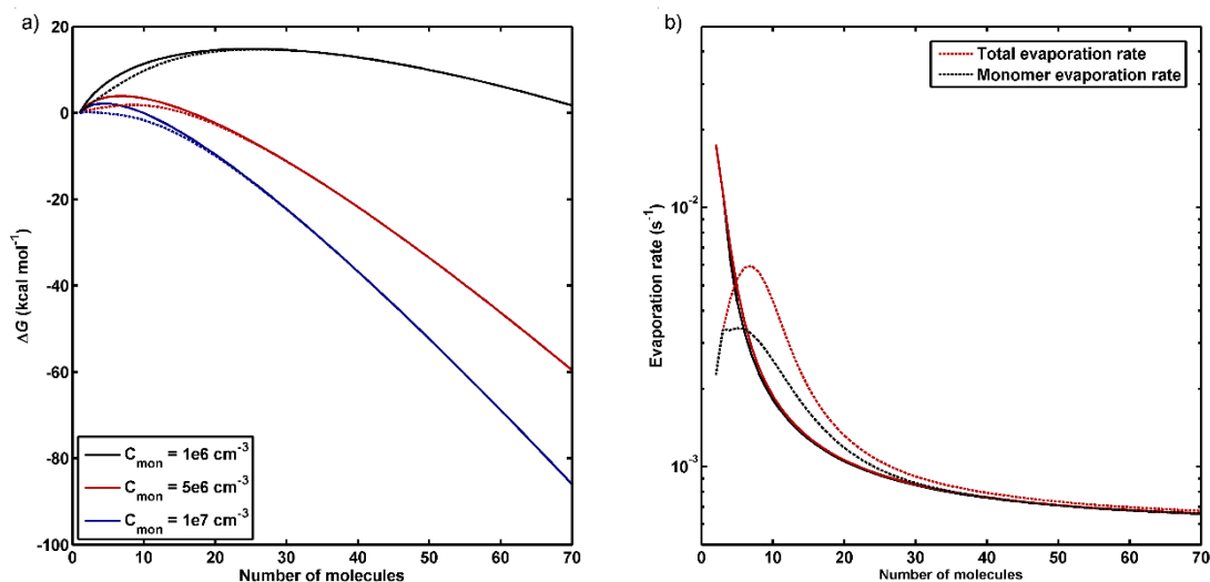
Figure A1. a) The classical Gibbs free energy profile with one maximum and no minima (solid lines) and with an additional negative term corresponding to stabilization of the smallest clusters (dashed lines) at different steady state monomer concentrations (shown as different colors). b) Evaporation profiles corresponding to the two Gibbs free energy profiles (note that the evaporation rate is independent of the vapor concentration).
