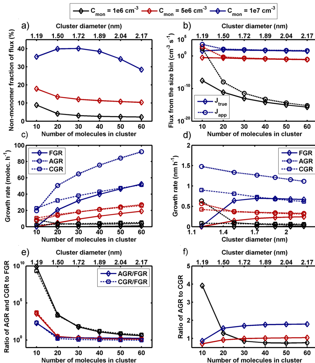
Figure 1. The effect of steady-state monomer concentration (shown as different colors) on quantities describing cluster growth: a) non-monomer fraction of flux from each size bin, b) the true collision-evaporation flux from each size bin ( J_{true} ; solid line) and the fluxes calculated from the appearance times of clusters ( J_{app} ; dashed line), c) and d) flux-equivalent growth rate (FGR; solid line), growth rate derived from the appearance times of clusters (AGR; dashed line), and growth rate calculated based on irreversible vapor condensation (CGR; dotted line), e) the ratios of AGR to FGR (solid line) and CGR to FGR (dotted line), f) the ratio of AGR to CGR.
