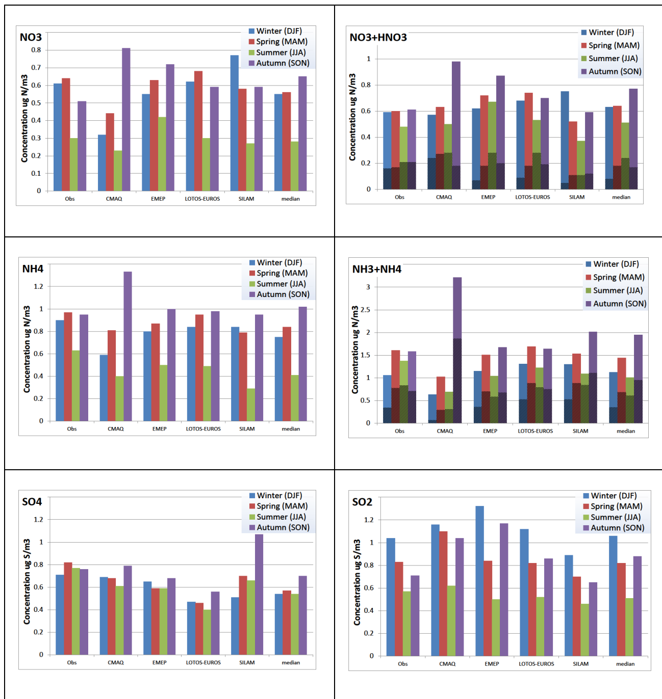
Figure 4. Observed and predicted seasonal concentrations of secondary inorganic aerosols and their precursors, mean over the EMEP stations [ \mu\text{g S/N m}^{-3} ]. Shaded part shows the concentration of the gas phase species \text{HNO}_3 and \text{NH}_3 . Only the stations where at least two of the gas, aerosol and their sum were observed, so that the gas phase fraction could be estimated, are included in the averaging. .
