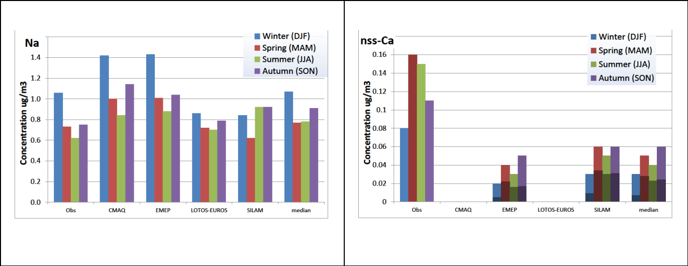
Figure 5. Observed and predicted seasonal concentrations of sodium and non-seasalt calcium in aerosol, mean over the EMEP stations [ \mu\text{g m}^{-3} ]. Modelled \text{Na}^+ concentrations are based on sea salt containing 30.8% \text{Na}^+ . Model values of non-sea-salt calcium assume 10% \text{Ca}^{2+} content of desert dust (shaded bottom part of the columns) and 3.5% calcium content of non-carbonaceous primary anthropogenic PM (the non-shaded upper part).
