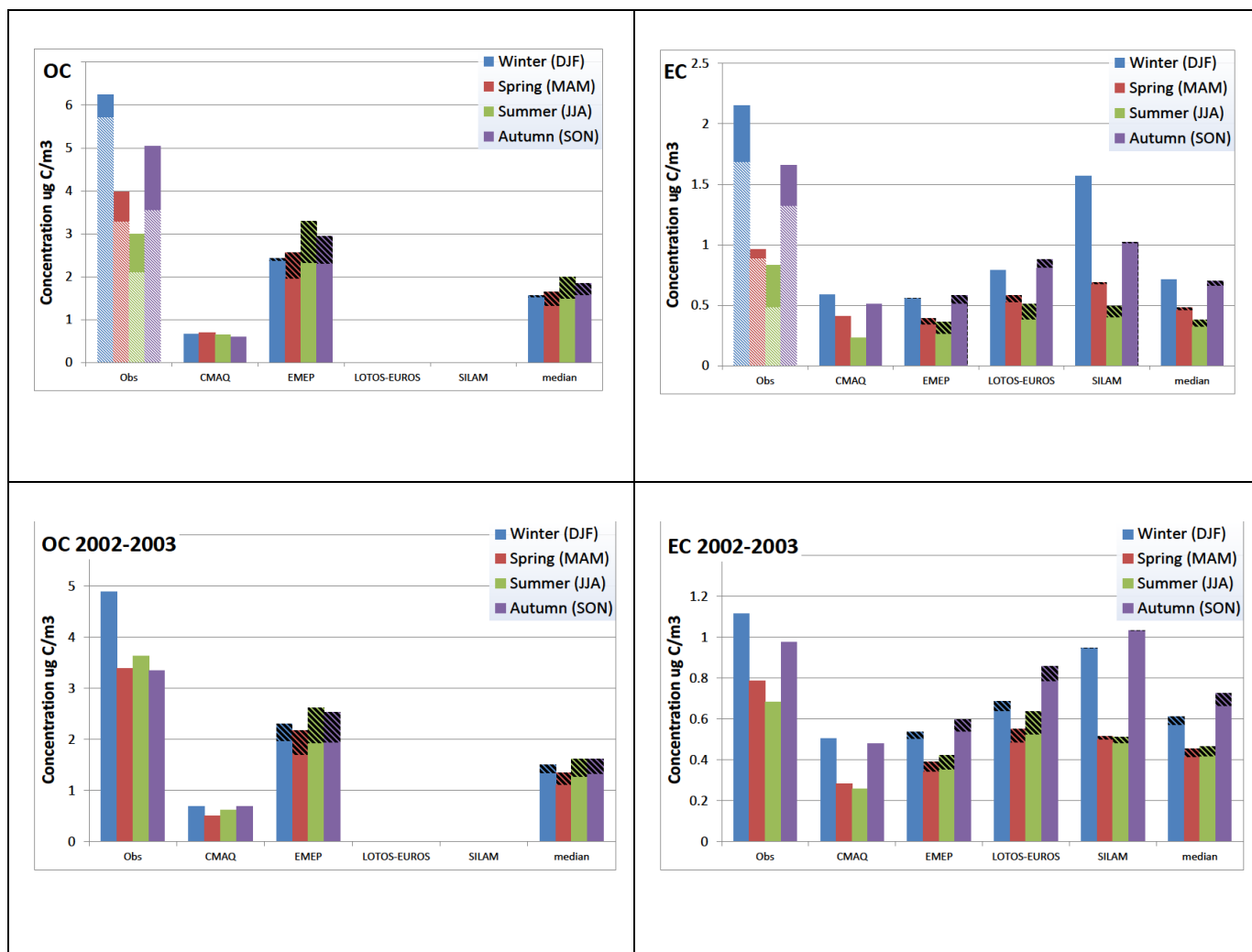
Figure 6. Observed and predicted seasonal concentrations of carbonaceous aerosols, mean over the EMEP stations [ \mu\text{g m}^{-3} ]. The panels on the left-hand and right-hand sides represent OC and EC, respectively. The upper row: 2005, data from 4 stations, for the observations the lighter shading marks the concentration in PM 2.5 , whole column the concentration in PM 10 ; the lower row: EMEP 2002-2003 campaign, observations of OC and EC in PM 10 . Dark shaded part shows the contribution from wild land fires (not separated for CMAQ OC, missing for CMAQ EC).
