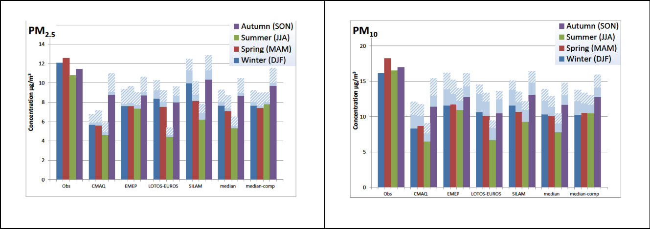
Figure 3. Observed and predicted seasonal concentrations of PM_{2.5} (left) and PM_{10} (right), mean over the EMEP stations [ \mu\text{g PM m}^{-3} ]. The light blue part shows the aerosol-bound water amount at the filter weighting conditions (50% relative humidity, 20°C), estimated with ISORROPIA2 based on the modelled aerosol composition. The solid light blue shows the water content in stable case (the lower curve of the hysteresis loop) and the striped part in metastable case (the upper branch of the hysteresis loop), when the crystallization has not occurred to aerosol coming from more humid conditions.
