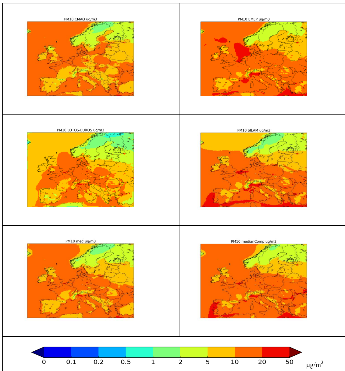
Figure 2. Annual mean dry PM 10 concentration predicted by the models, their median and medianComp [ \mu\text{g PM m}^{-3} ]. The dots show the annual mean observed values in EMEP stations (only the stations with observations available for at least 75% of the time are shown).
