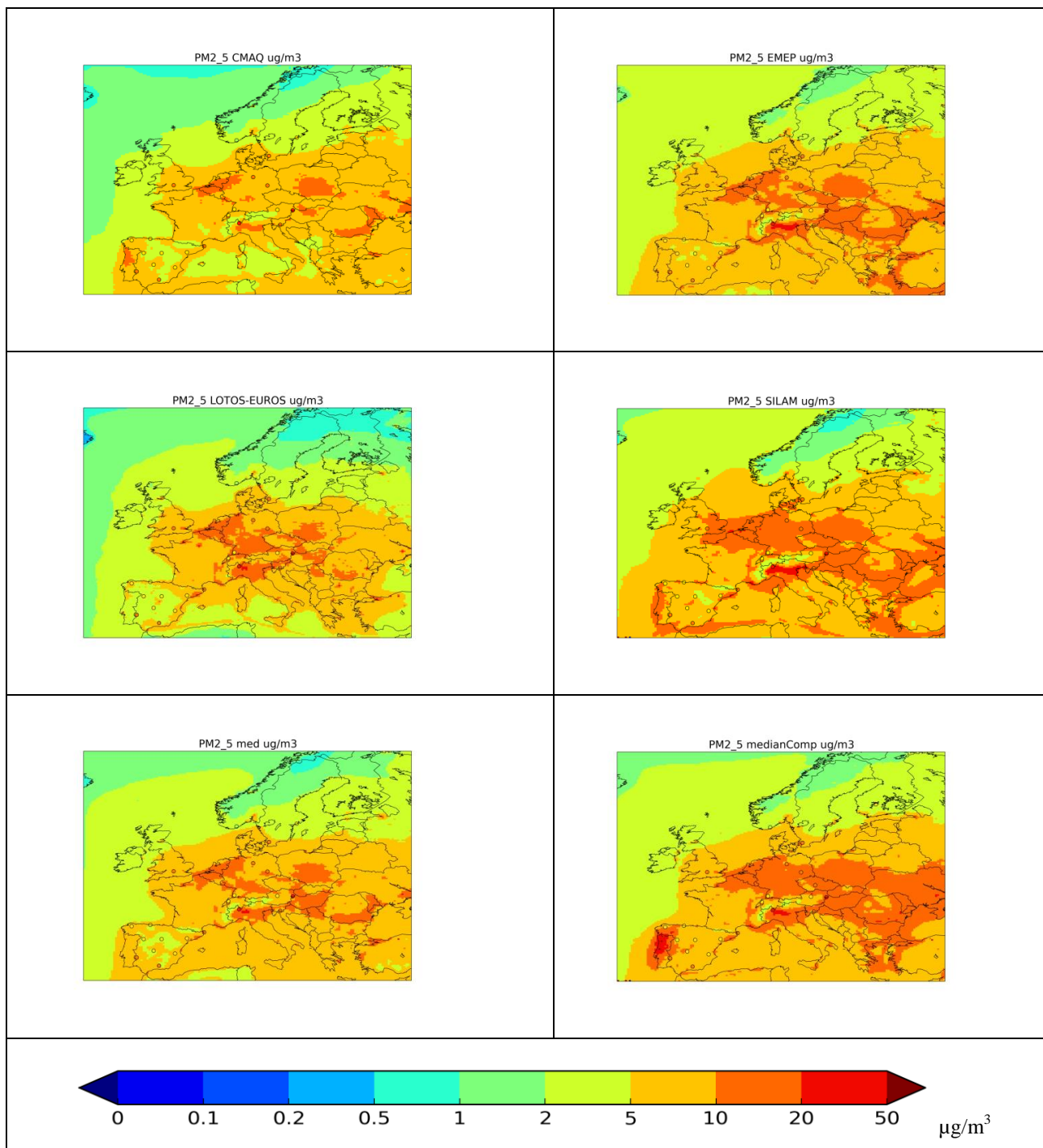
Figure 1. Annual mean dry PM 2.5 concentration predicted by the models, their median and medianComp [ \mu\text{g PM m}^{-3} ]. The dots show the annual mean observed values in EMEP stations (only the stations with observations available for at least 75% of the time are shown)
