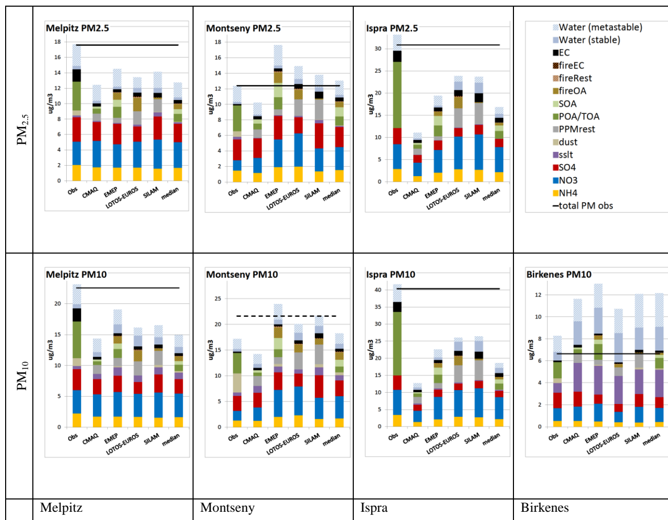
Figure 8. Aerosol chemical composition measured and modelled at four stations. Upper row – PM 2.5 , lower row – PM 10
