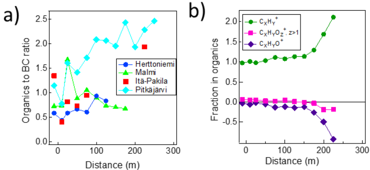
Figure 5. The average ratio of organics to BC at four sites (a) and the fractions of hydrocarbon fragments ( C_xH_y^+ ) and oxidized organic fragments ( C_xH_yO^+ and C_xH_yO_z^+, z>1 ) at Pitkäjärvi (b) as a function of the distance from the highway. Zero distance refers to the roadside and negative value driving on the highway. Background values were subtracted from the measured concentrations before calculating the ratios.
