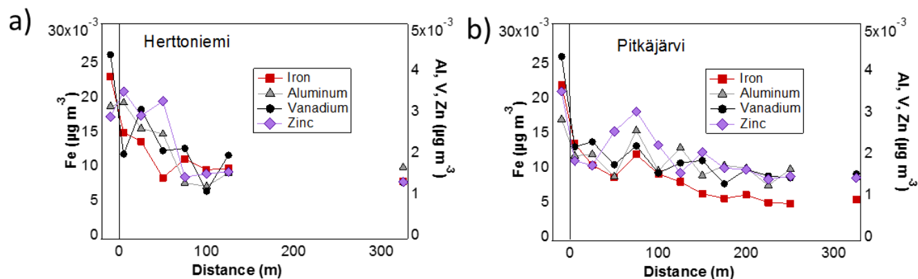
Figure 8. Concentrations of iron, aluminum, vanadium and zinc at Herttoniemi (a) and Pitkäjärvi (b) as a function of the 5 distance from the highway. Zero distance refers to the roadside, negative values to driving on the highway and right-most point to the background location. Background values are not subtracted from the measured concentrations. Gradients for Itä- Pakila and Malmi are presented in supplement.
