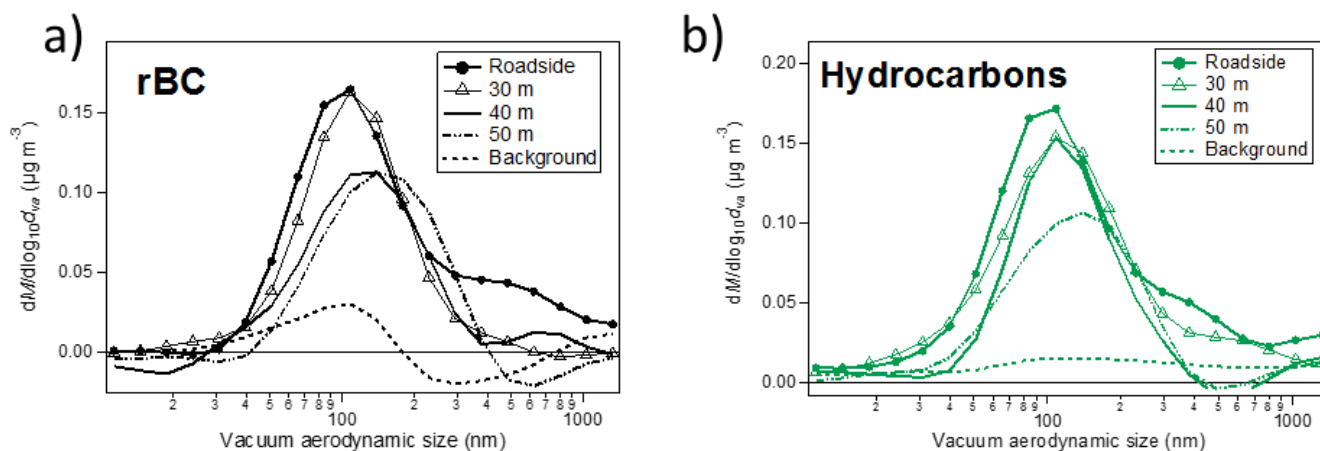
Figure 7. Particle mass size distribution at Herttoniemi on 26th of Oct 2012. m/z 36 was used as a surrogate for rBC and m/z 57 for for hydrocarbons.
