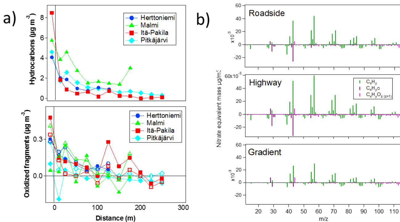
Figure 6. Concentrations of hydrocarbon fragments ( \text{C}_x\text{H}_y^+ ) and oxidized organic fragments ( \text{C}_x\text{H}_y\text{O}^+ and \text{C}_x\text{H}_y\text{O}_z^+ , z > 1 ) measured at the four sites (a), and the average mass spectra for highway, roadside and gradient at Pitkäjärvi (b). Solid markers refer to organic fragments with one oxygen atom and open markers to organic fragments with more than one oxygen atoms in lower figure of (a). In (a) zero distance refers to the roadside and negative value driving on the highway. Background values were subtracted both from the measured concentrations and mass spectra.
