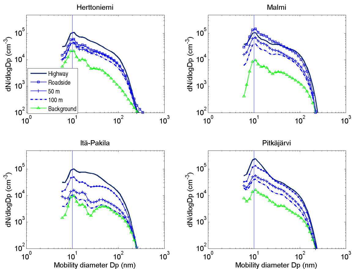
Figure 3. Particle size distribution as measured by the EEPS at different distances from the roadside on the four locations.
