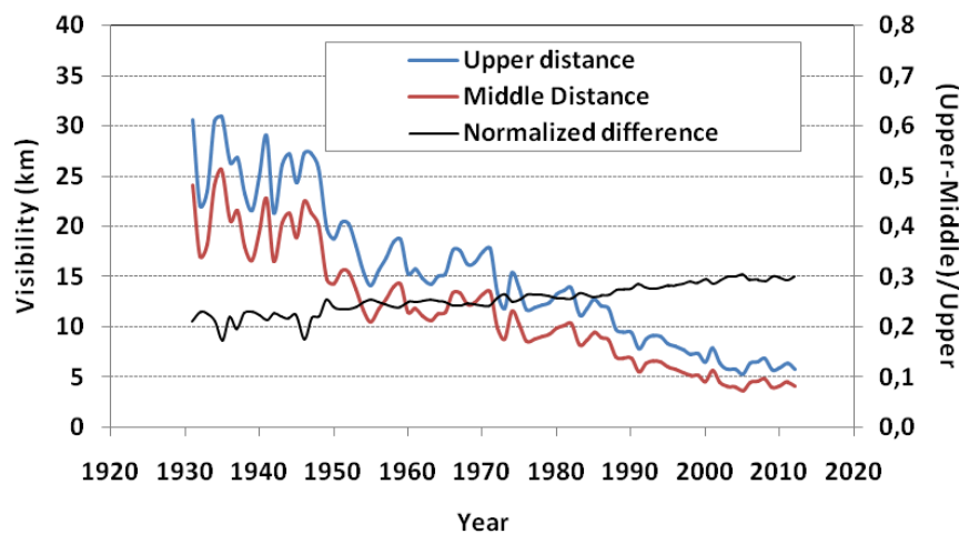
Figure S3: Variation of the annual visibility at NOA from 1931-2013, estimated from the upper distance (blue line) and the middle distance (red line) in the ranges of WMO scale (Table 2 of the manuscript). The black line illustrates the relative difference between the two time series.
