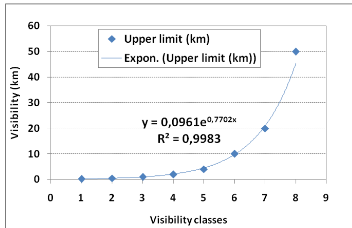
Figure S1: Relationship between the upper distance of visibility ranges and visibility classes in WMO scale (Table 2 of the manuscript).
