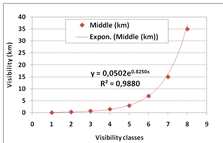
Figure S2: Relationship between the middle distance of visibility ranges and visibility classes in WMO scale (Table 2 of the manuscript).
