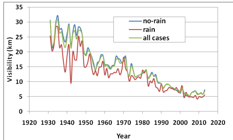
Figure S4: Variation of visibility at NOA from 1931-2013, estimated from subsets of ‘rain’ and ‘no-rain’ days as well as the ‘all cases’ set. A rainy day is defined as a day with total precipitation > 1\text{mm} , following WMO.
