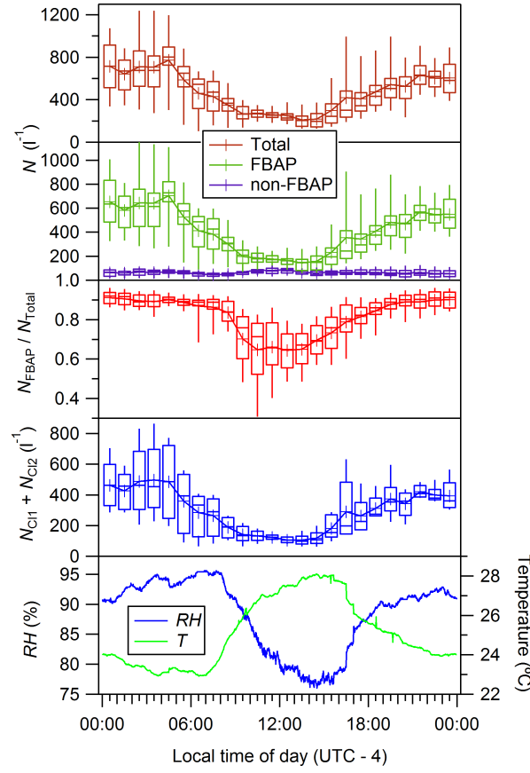
Figure 9. Diurnal variations in total, FBAP and non-FBAP number concentrations, as measured by the WIBS-3M, as well as the fraction of FBAP, and the combined number concentrations of clusters C11 and C12. Shown are the means (lines and markers), medians and inter-quartile ranges (boxes) and 5th and 95th percentiles (whiskers). Also shown at the bottom are the mean diurnal variations in temperature and RH , measured on the tower above the canopy, for the same period.
