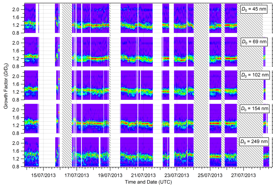
Figure 7. The time-series of normalised RH -corrected (to 90%) growth factor distributions derived from HTDMA measurements, for all 5 dry diameters. Shaded areas represent pollution episodes removed from the data. Any other gaps are due to instrument down-time and humidograms.
