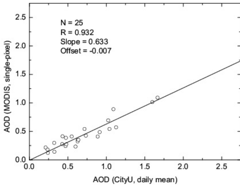
Fig. 8. MODIS single-pixel AOD versus sun-sky radiometer daily mean AOD.
