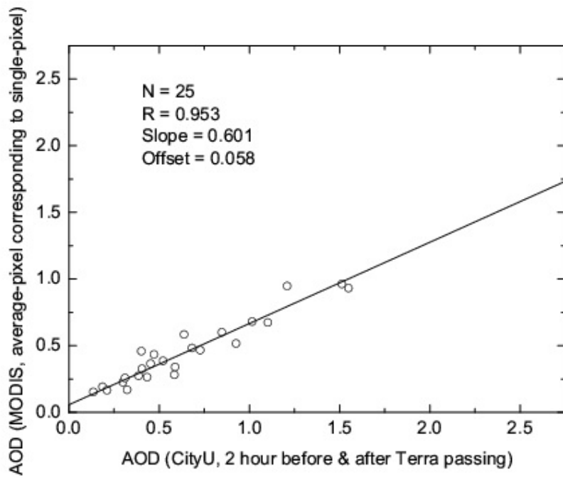
Fig. 6. MODIS mean-pixel AOD corresponding to the single-pixel data at the same day as in Figure 5 versus sun-sky radiometer mean AOD 2-hour before and after Terra passing.
