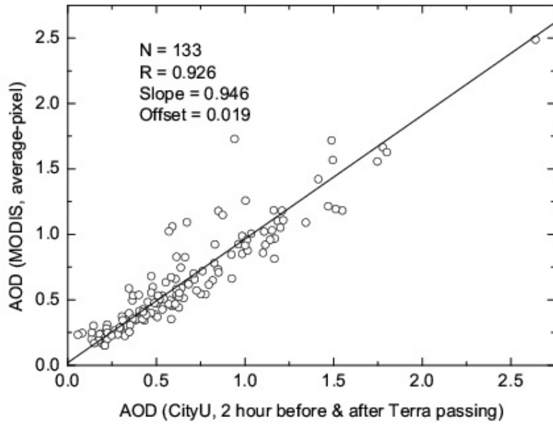
Fig. 4. MODIS mean-pixel AOD versus sun-sky radiometer mean AOD 2-hour before and after Terra passing.
