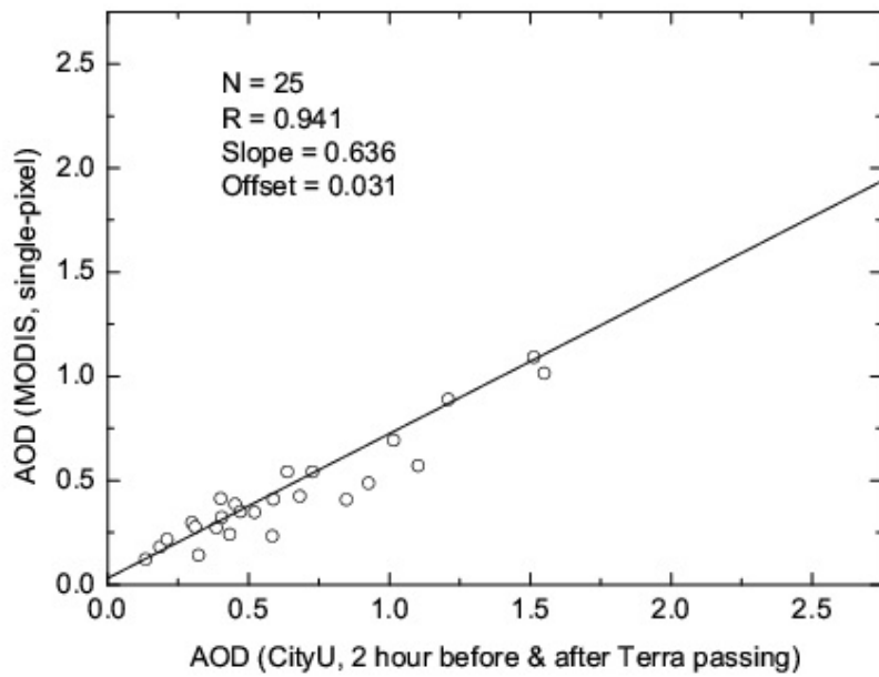
Fig. 5. MODIS single-pixel AOD versus sun-sky radiometer mean AOD 2-hour before and after Terra passing.
