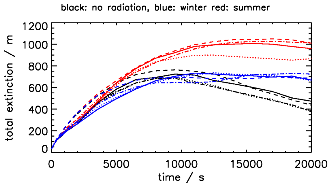
Fig. 1. Temporal evolution of total extinction. Each simulation (as denoted by colour coding on top) was run with 4 different initial turbulence fields, denoted by the various linestyles of the curves.
