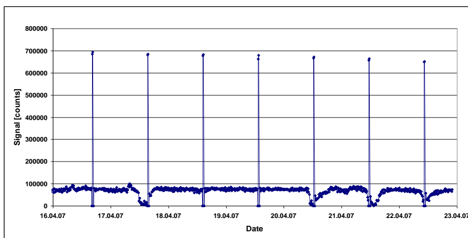
Fig. 1: Raw signal of the Tekran instrument at Cape Point in April 16-22, 2007. Note that the automatic calibrations on April 17, 20, 21, and 22 coincide with the DEs.
