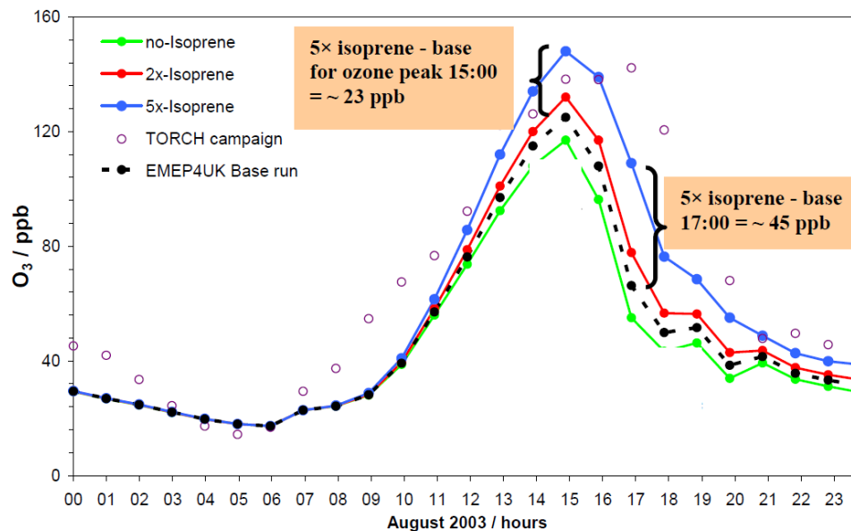
Fig. 2. 6th of August 2003 ozone concentration.
