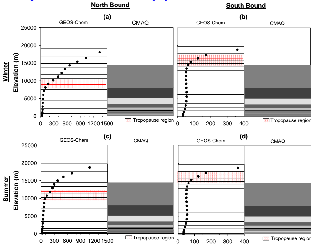
Fig. 5. Vertical ozone profiles from GEOS-Chem with CMAQ layers for both summer and winter, (a) north bound in winter, (b) south bound in winter, (c) north bound in summer, and (d) south bound in summer
