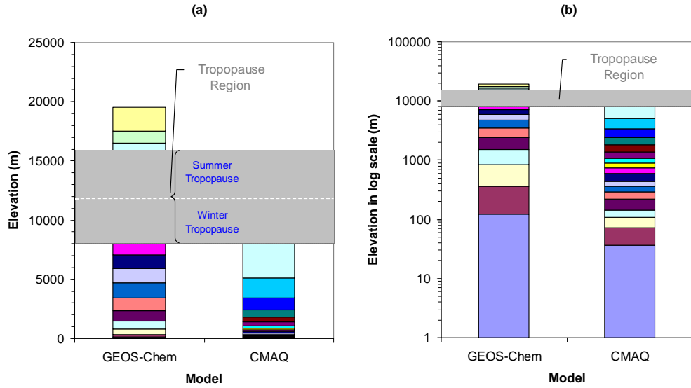
Fig. 1. Vertical layer structure comparison between GEOS-Chem and CMAQ, (a) arithmetic scale, and (b) log scale
