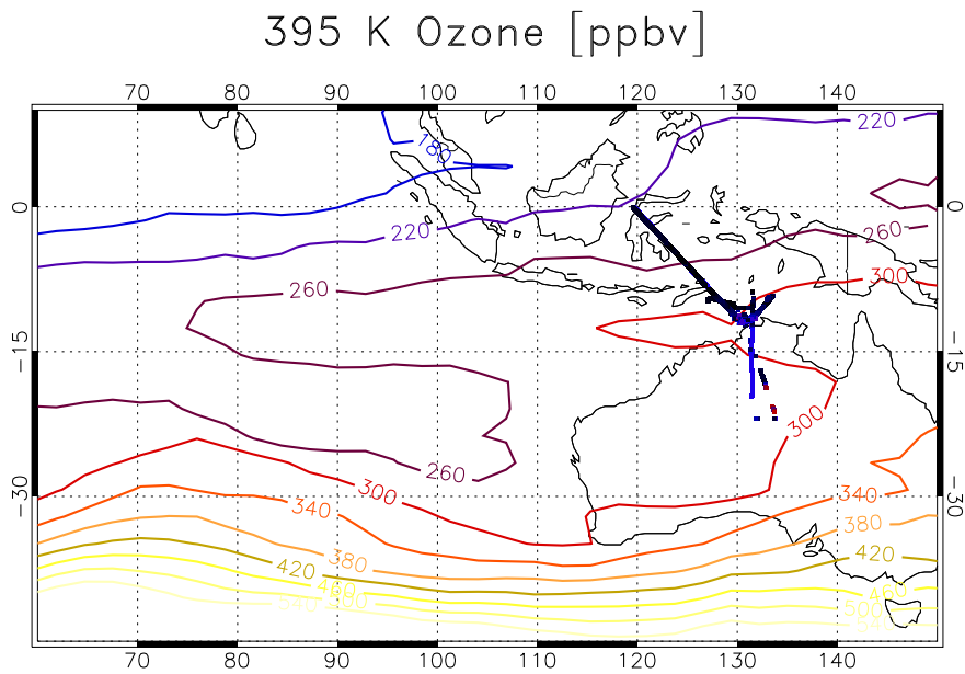
Fig. 3. O 3 model field at 395 K with superimposed the measured O 3 mixing ratios (same color code), for the SCOUT-Darwin campaign.
