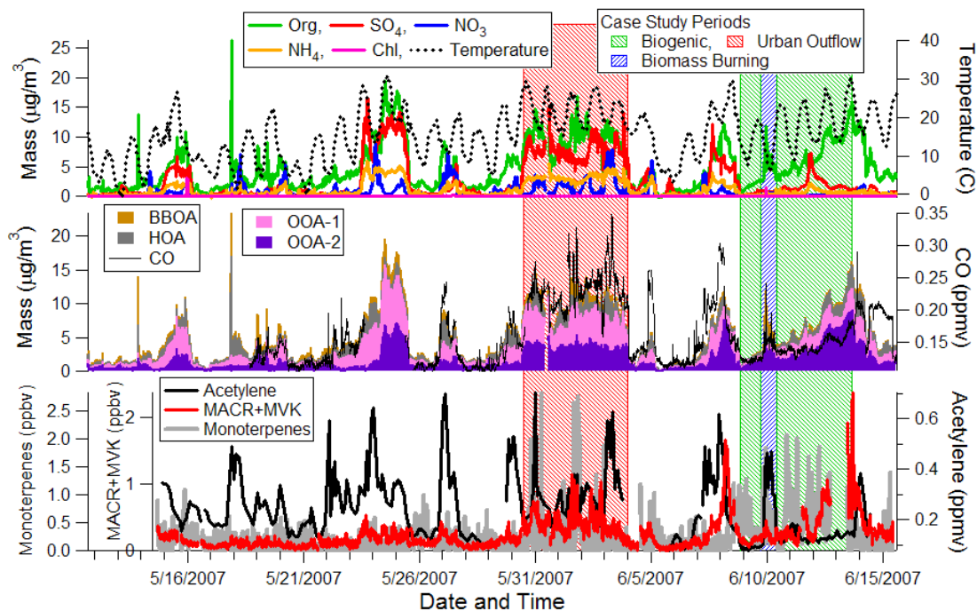
Fig. 1. Time series of AMS measurements (top panel), AMS PMF factors (middle panel), and selected gas-phase species (bottom panel).
