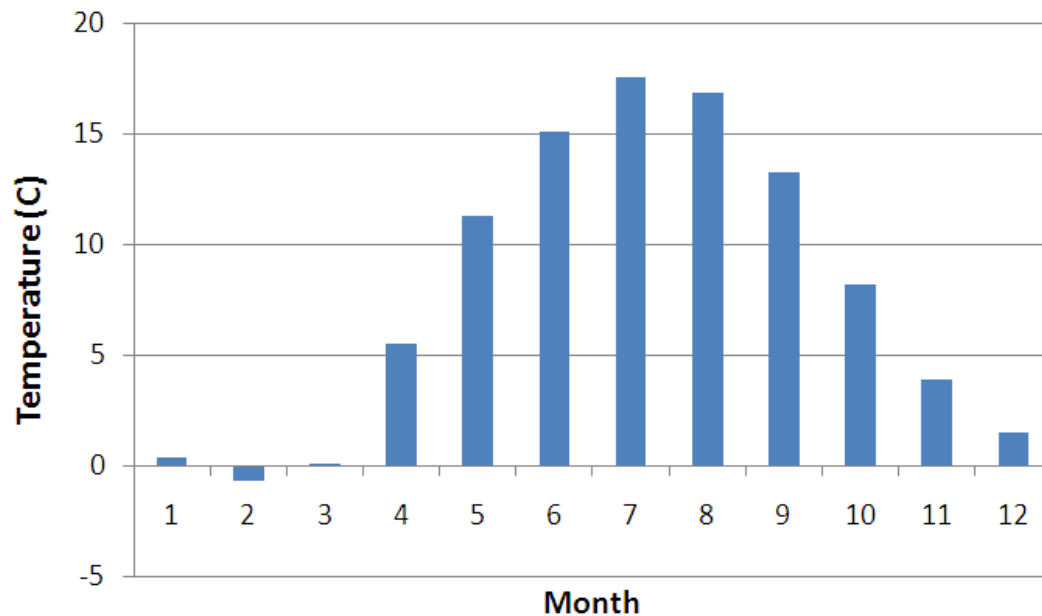
Fig. 3. Monthly temperature in 2005 in Europe.
