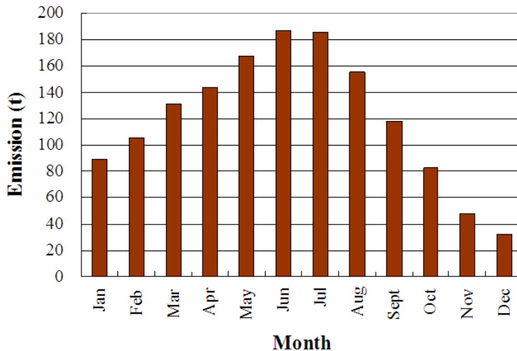
Fig. 1. Monthly emission of gamma-HCH for 2005.
