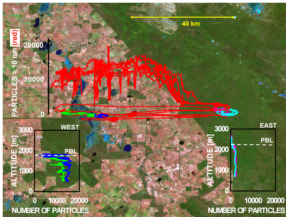
Fig. 2. Fig. 2: Flight patterns crossing the State Barrier Fence, 9.12.07, summer season, Number of ultrafine particles ( > 10 nm, red) on six horizontal flight legs, and vertical profiles east and west of the
