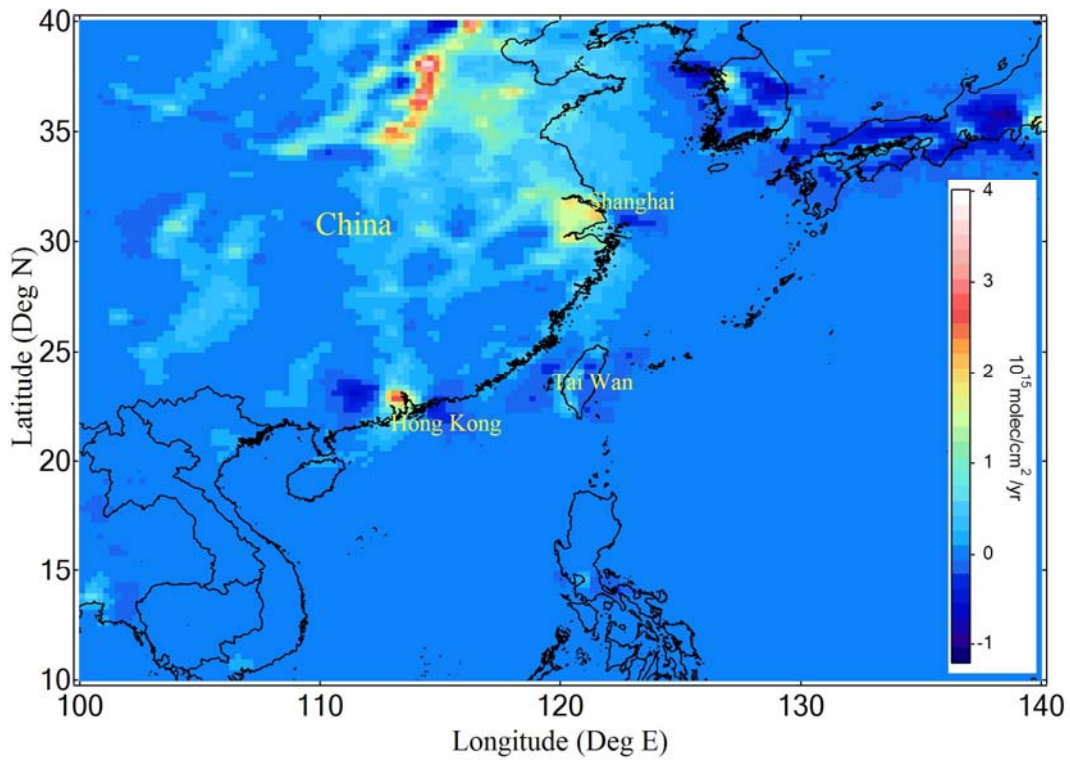
The trend of tropospheric NO 2 column during (1996-2007)
