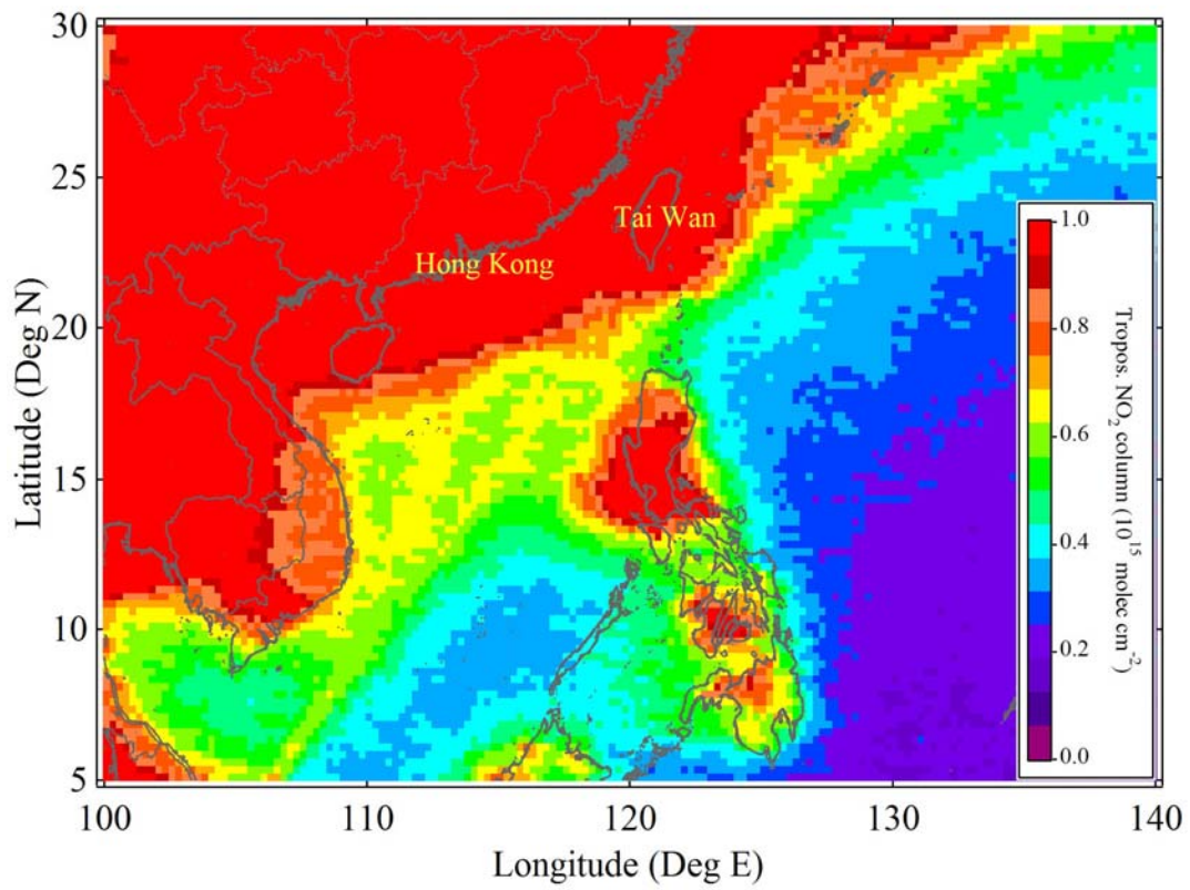
Mean tropospheric NO 2 column over the ocean showing the main shipping routes in SE China
