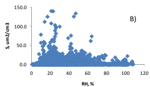
Figure 2. Surface area concentration versus RH at Izaña.
