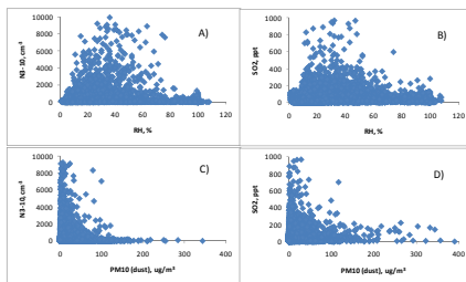
Figure 3. Hourly concentrations of N3-10 and SO2 versus PM10 and RH at Izaña.
