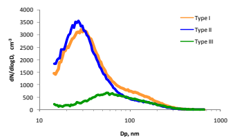
Figure 1. Size distribution during Type I events (when N13-20 and SO 2 were correlated and N13-10 > 100 cm -3 ), Type II events (when N13-20 and SO 2 were not correlated and N13-10 > 100 cm -3 ), and Type III events (N13-10 < 100 cm -3 ).
