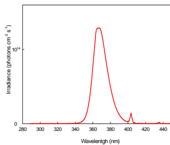
Spectral irradiance of the UV-A lamps used in the flow tube experiments tube. The total irradiance in the 300–420 nm range is 1.8 \times 10^{15} photons \text{cm}^{-2} \text{s}^{-1} .
