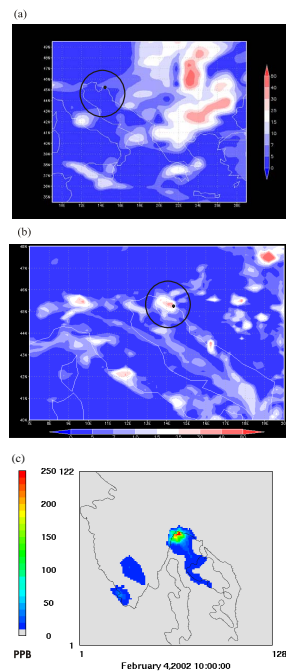
Appendix 1: The horizontal distribution of hourly surface EMEP SO 2 concentrations on 4 February 2002 at 10:00 UTC (a) with 50-km EMEP model (µgS m -3 ); (b) with 10-km EMEP4HR model (µgS m -3 ); and, (c) with 1-km CAMx model over the greater Rijeka area domain (ppb). The black circles and black dots at two upper panels display the studied area (north-eastern Adriatic) and the position of Rijeka town, respectively. The emissions at 1x1 km 2 horizontal resolution (for CAMx) were obtained by interpolation from 10 x10 km 2 .
