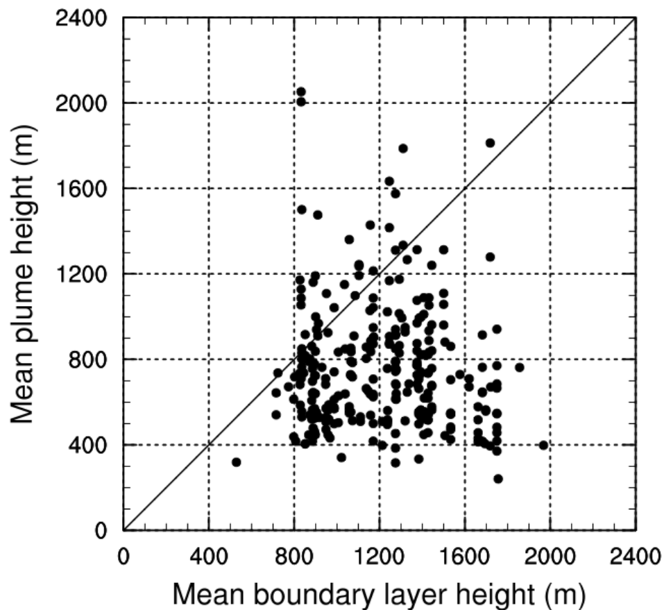
Fig. 1. (Figure R1): Observed mean plume heights (MISR) v. mean boundary layer heights (GEOS) for Borneo 2001–2006.
