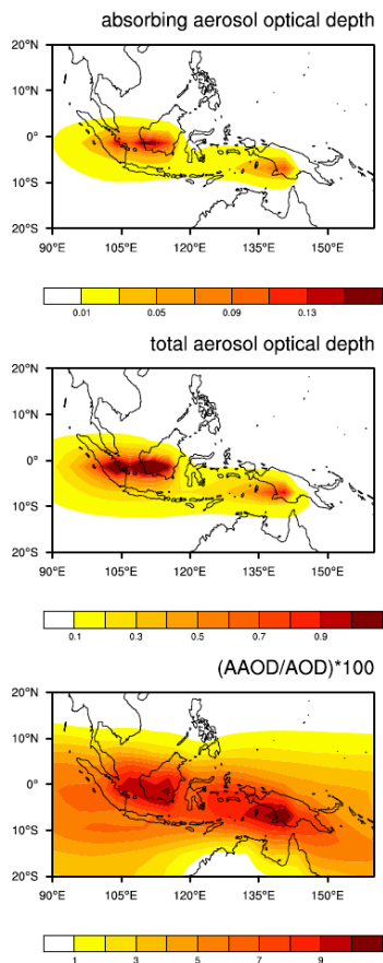
Fig. 2. (Figure R2): Simulated high fire minus low fire absorbing aerosol optical depth (top), total aerosol optical depth (middle) and percent increase in optical depth due to absorbing aerosols (bottom).
