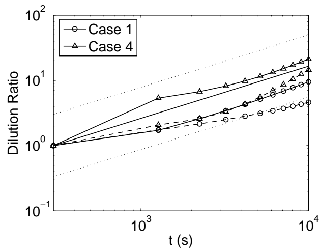
Figure 1: Dilution ratio plotted against time relative to the plume dilution at t = 300 seconds. The SPM dilution (solid, symbols) and Konopka (1995) model dilution (dashed, symbols) are plotted for case 1 and case 4 as in Figure 5. The mean data fit from Schumann et al. (1998) is plotted (solid) along with a factor of 3 scatter range (dotted).
