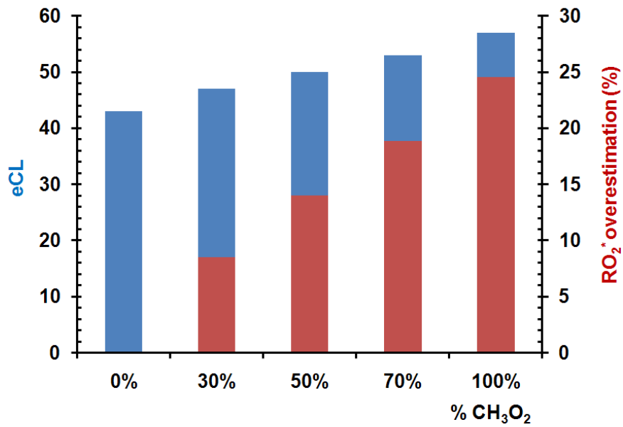
Figure 4411: Simulated eCL values for different HO 2 and CH 3 O 2 mixtures (0% implies a pure HO 2 sample). Red bars represent the corresponding overestimation in the RO 2 * mixing ratios determined with the eCL for HO 2 .
