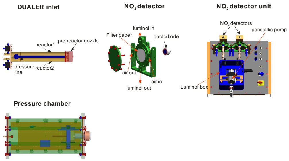
Figure 1: Schematic presentation of the instrumental set up used for characterisation experiments and detail of some of the components of the IUP-UB DUALER.
