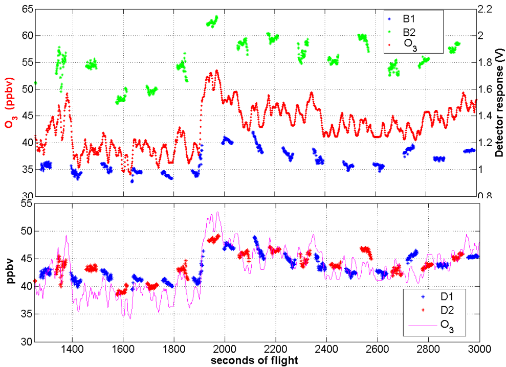
Figure 12: Example of calculation of effective calibration parameters on the basis of O 3 DLR-Falcon measurements at 330 mbar on the 13 August 2006 (900 data points) a) comparison between [O 3 ] in ppbv and background volt signals of the luminol detectors (B1 and B2 respectively), b) D1 and D2 detector signals in ppbv calculated with the obtained calibration parameters ( A_{\text{Det1}}=28.2\pm4.5 ; A_{\text{Det2}}=16.8\pm3.1 ; B_{\text{Det1}}=16.9\pm1.9 ; B_{\text{Det2}}=14.3\pm1.5 ).
