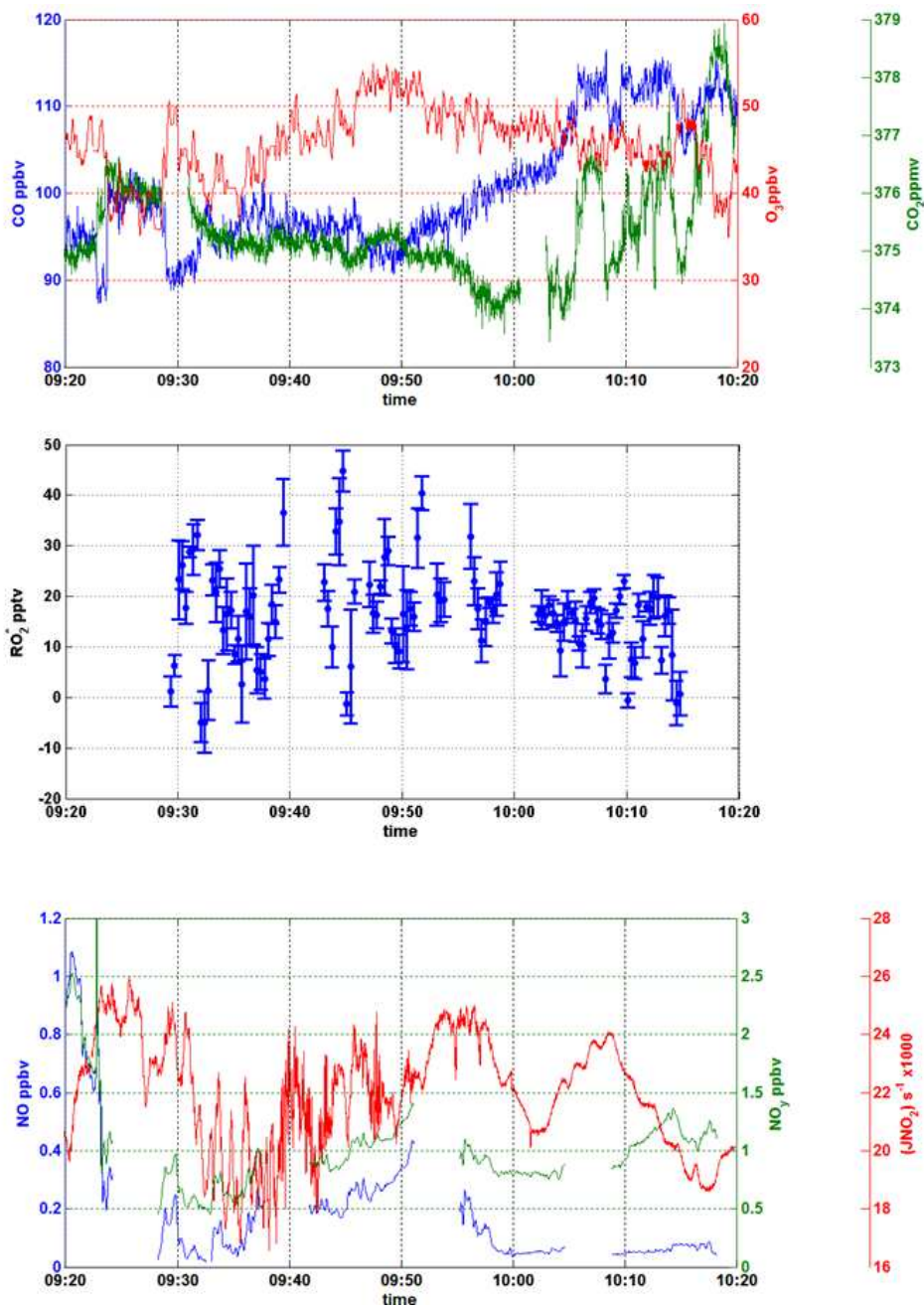
Figure 16134: Mixing ratios measured on the 4 August 2006 at 315 mbar. The [RO 2 * ] error bars represent the statistical error of the 20s averages. The total [RO 2 * ] error remains around 25% (see text).
