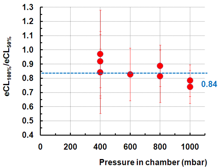
Figure 4310: Variation with the pressure of the ratio between eCL s obtained for 100% HO 2 (indicated as eCL_{100\%} ) and for a mixture of 50% HO 2 plus 50% CH 3 O 2 (indicated as eCL_{50\%} ). The mean ratio is 0.84.
