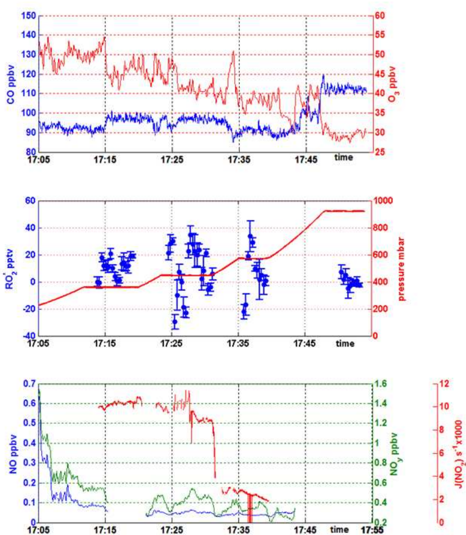
Figure 45123: Mixing ratios measured on the 11 August 2006 within a vertical profile taken between 360 and 960 mbar. The [RO_2^*] error bars represent the statistical error of the 20s averages. The total [RO_2^*] error remains below 45% (see text).
