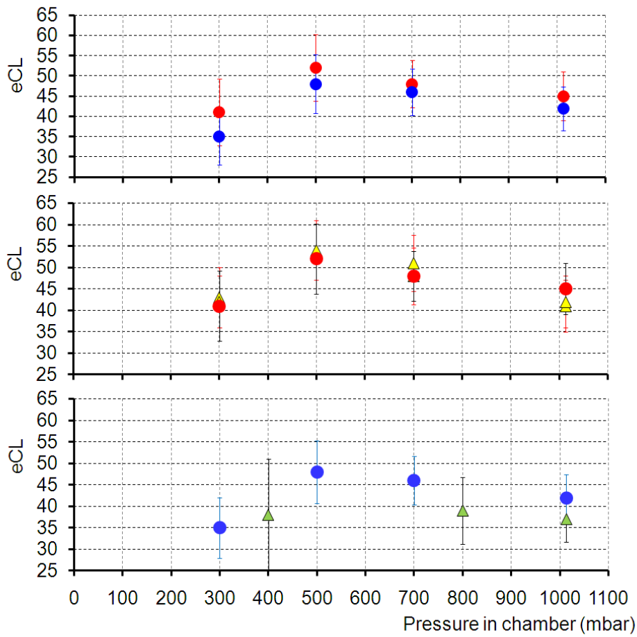
Figure 86: Variation of the eCL with the ambient pressure for the DUALER a) without pressure regulation, b) regulated at 200 mbar and c) regulated at 300 mbar. The eCL obtained without pressure regulation is also plotted in b) and c) for comparison (red dots: reactor 1; blue dots: reactor 2). Det. i : detector i
