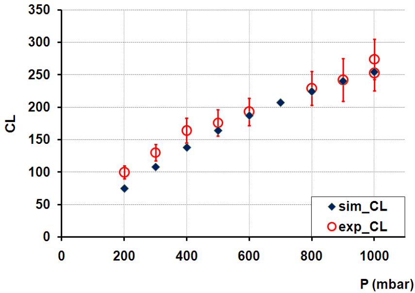
Figure 64: Variation of the CL with the pressure as measured for a single reactor. Simulated (sim-CL) and experimental CL (exp_CL) are plotted for comparison.
