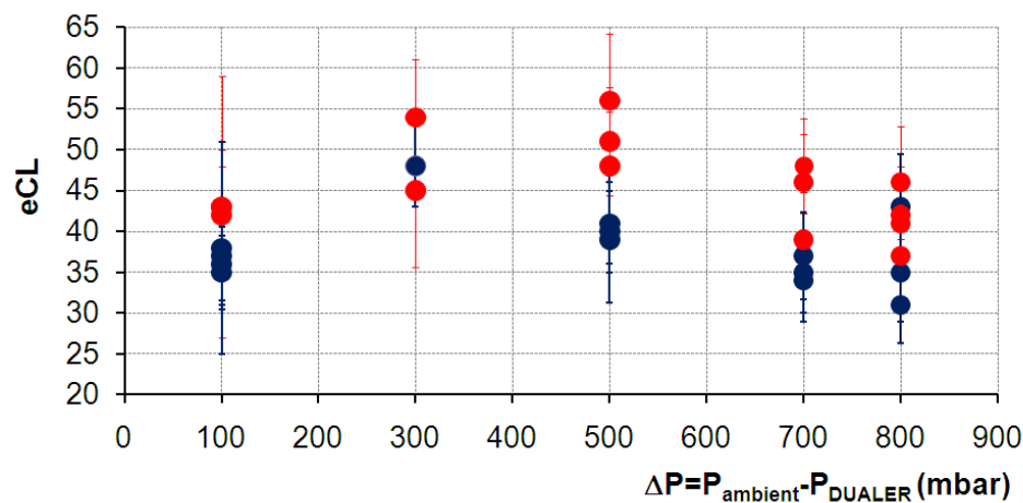
Figure 107: Experimental eCL values obtained for different \Delta P = P_{\text{ambient}} - P_{\text{DUALER}} . The DUALER is kept at 200 mbar. In red eCL for reactor 1 and in blue for reactor 2.
