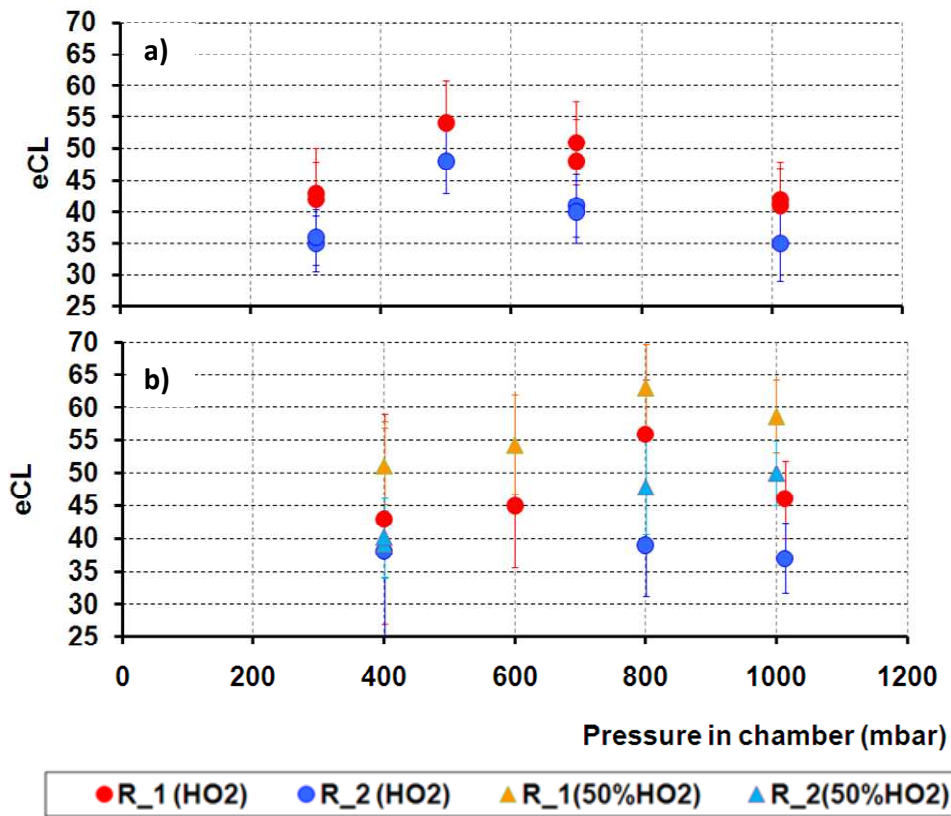
Figure 75: Variation of the eCL with the ambient pressure. The IUP-DUALER is kept at a constant pressure: a) 200_mbar, b) 300 mbar. R_i (50% HO 2 ) corresponds with a 50% HO 2 /50% CH 3 O 2 radical mixture for reactor i . R_i (XO 2 ): for reactor i and peroxy radical XO 2 .
