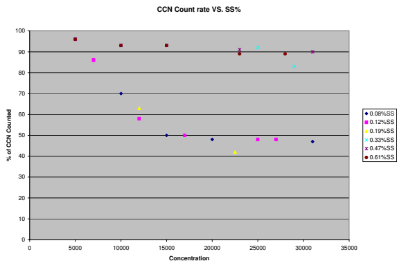
Figure 28. CCN Count Rate VS. SS%
