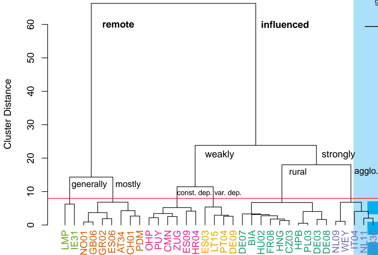
Fig. 1. Clustering dendrogram for site categorisation.
