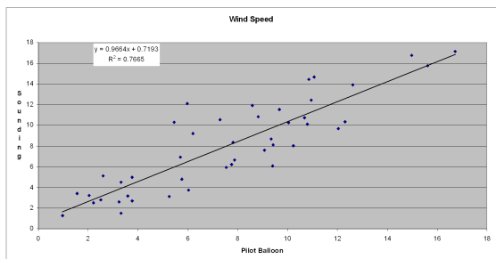
Wind speed correlation between soundings and pilot balloons
