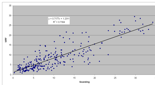
Wind speed correlation between Soundings and WRF model simulations
