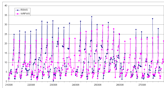
Wind speed vertical profiles for Soundings and WRF model simulations
