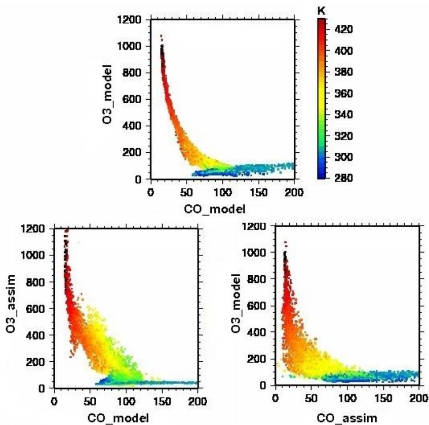
Fig. 1. Top: Modelled O 3 Vs modelled CO; Left: Assimilated O 3 Vs modelled CO; Right: Modelled O 3 Vs assimilated CO. The colour code is the same and refers to the potential temperature in K. O 3 & CO are in ppb
