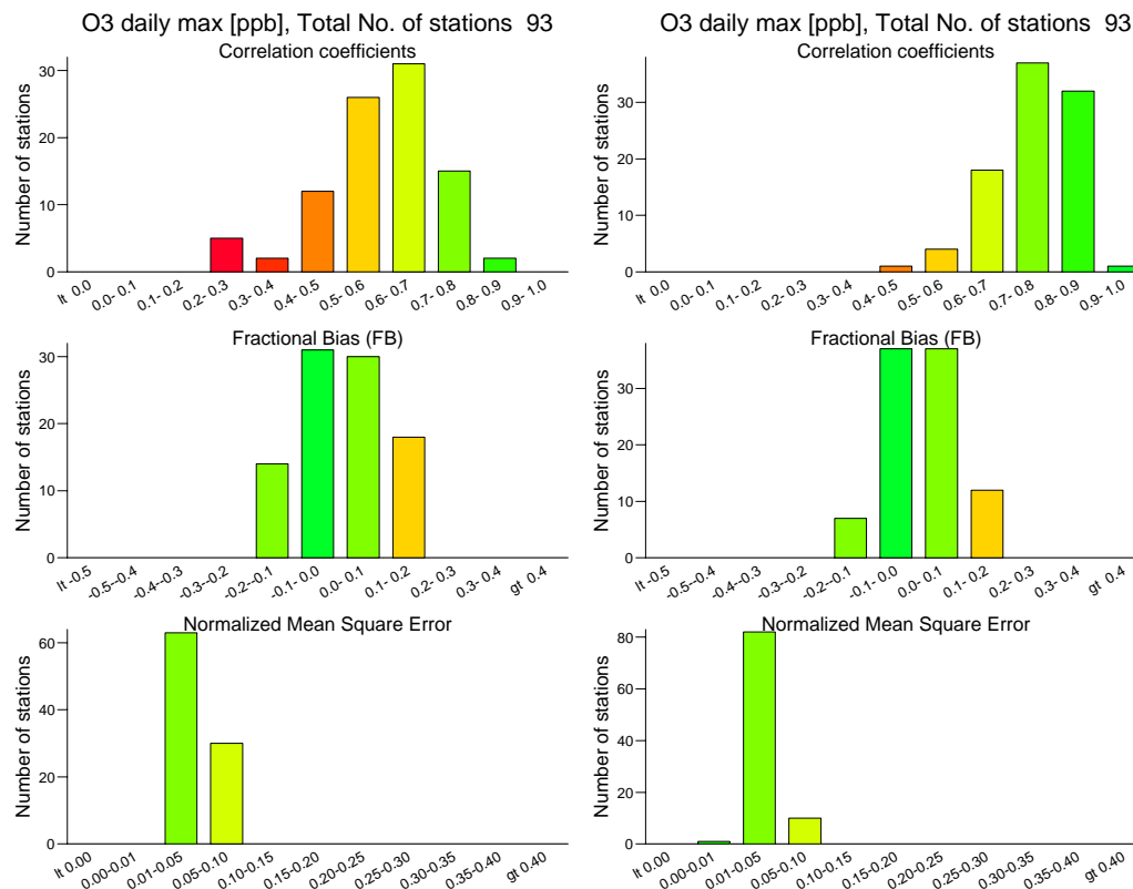
Fig. 4. Frequency distributions for the correlation coefficient, the fractional bias and the normalized mean square error, including the statistics from comparisons between measurements and model results for the daily maximum values at each measurement stations within the EMEP network. The testing period is April–September 1999. The upper figure shows the results from the reference run without applying the data assimilation technique. The lower figure shows the results from a model run including the data assimilation as the configuration in experiment 8.
