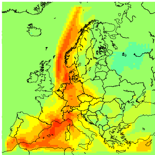
Fig. 10. Daily maximum ozone concentrations calculated using DEOM during an ozone episode in Europe in 12 September 1999. The upper figure shows the results from the reference run without using data assimilation. The lower figure shows the corresponding result including the data assimilation of surface O 3 based on the configuration in experiment 8.
