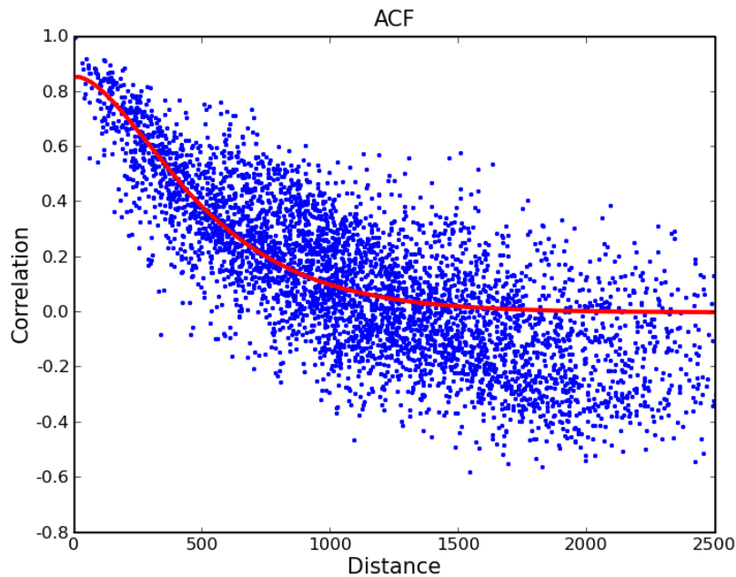
Fig. 1. The correlation function Eq. (3) is fitted to the departures correlation as a function of the distance between them in km.
