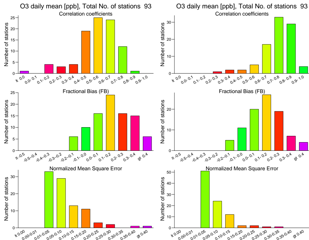
Fig. 3. Frequency distributions for the correlation coefficient, the fractional bias and the normalized mean square error, including the statistics from comparisons between measurements and model results for the daily mean values at each measurement stations within the EMEP network. The testing period is April–September 1999. The upper figure shows the results from the reference run without applying the data assimilation technique. The lower figure shows the results from a model run including the data assimilation as the configuration in experiment 8.
