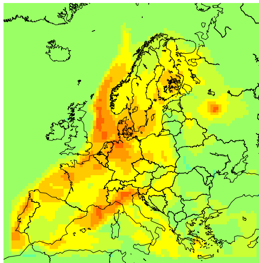
Fig. 9. Daily maximum ozone concentrations calculated using DEOM during an ozone episode in Europe in 7 September 1999. The upper figure shows the results from the reference run without using data assimilation. The lower figure shows the corresponding result including the data assimilation of surface O 3 based on the configuration in experiment 8.
