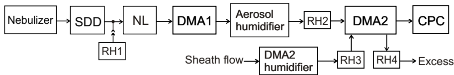
Fig. 1. Experimental setup of the hygroscopicity tandem differential mobility analyzer (H-TDMA) system: RH – relative humidity sensor, SDD – silica gel diffusion dryer, NL – aerosol neutralizer, DMA – differential mobility analyzer, CPC – condensation particle counter.
